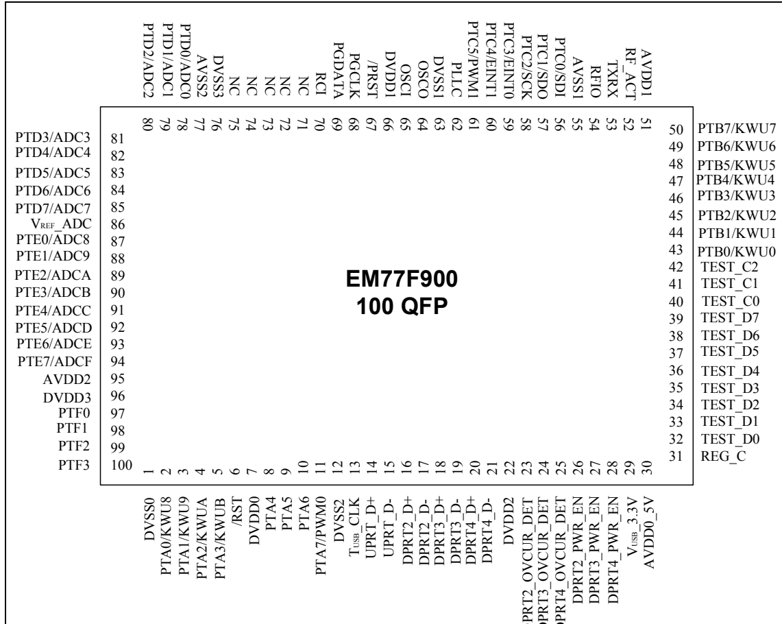
Fig. 3-1 Pad and Pin Configuration of EM77F900
