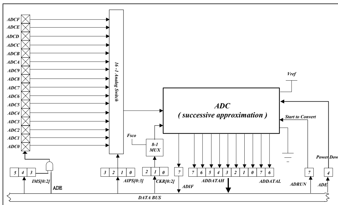
Fig 11-1 Analog-to-Digital Conversion Functional Block Diagram
