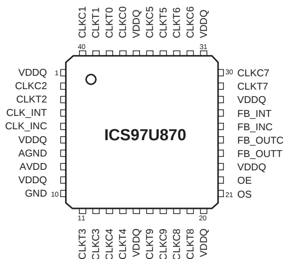
40-Pin MLF
