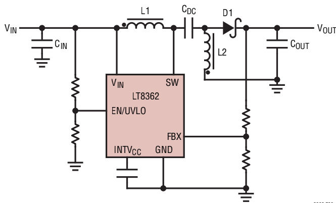
Figure 6. LT8362 Configured in a SEPIC Topology
