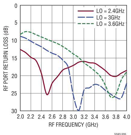
Figure 5. RF Port Return Loss
