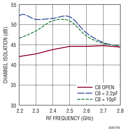
Figure 4. Channel-to-Channel Isolation vs C8 Values
