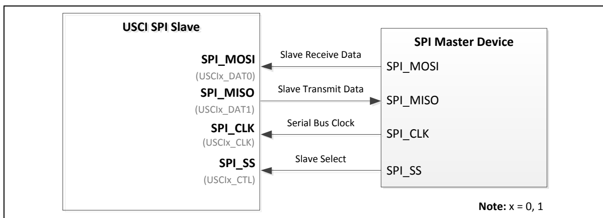
Figure 6.27-2 SPI Slave Mode Application Block Diagram
