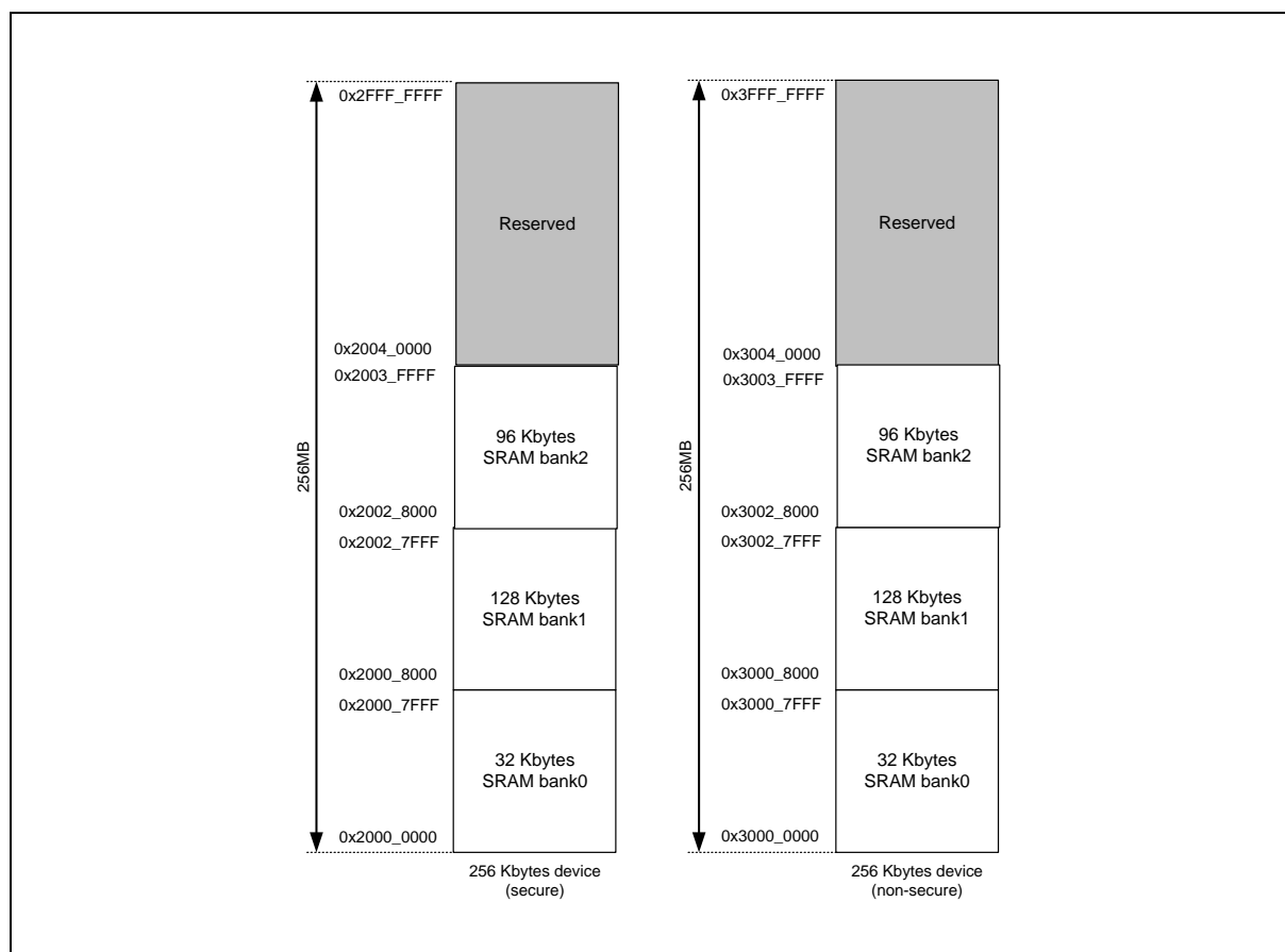
Figure 6.2-11 SRAM Memory Organization
