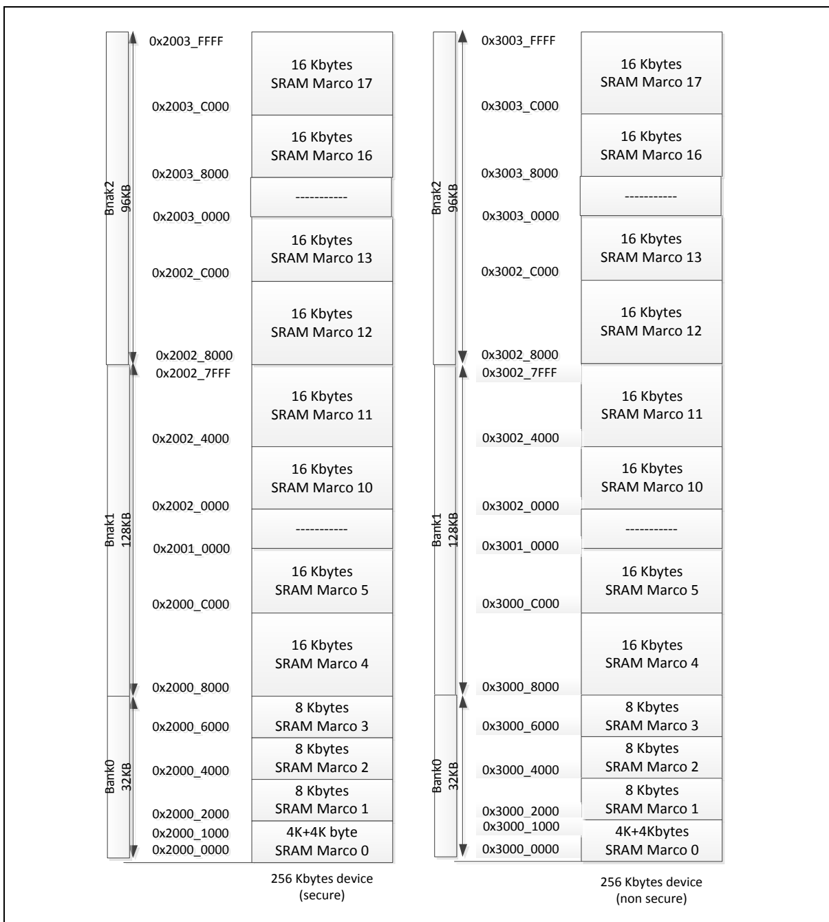
Figure 6.2-12 SRAM Marco Organization
