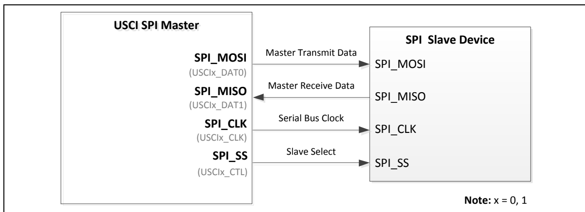
Figure 6.27-1 SPI Master Mode Application Block Diagram
