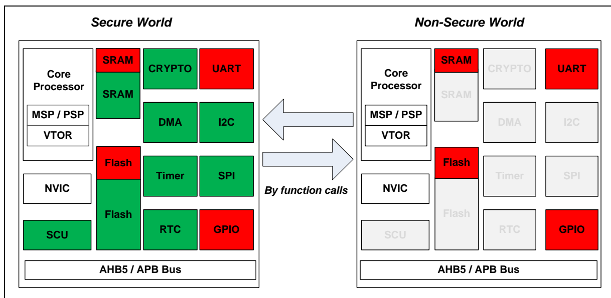
Figure 6.5-1 Secure World View and Non-secure World View on a Chip
