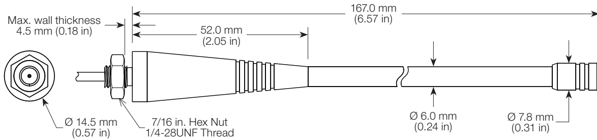
Figure 6. PW 450 MHz Antenna Dimensions
