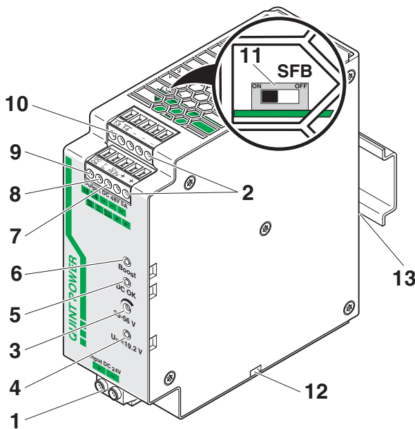
Figure 2 Function elements
