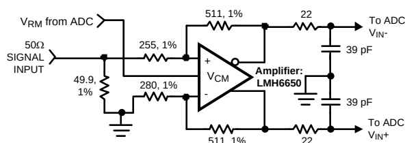
Figure 6. Optional Amplifier Drive for Circuit in Figure 5
