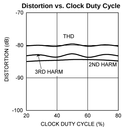
Distortion vs. Clock Duty Cycle (DCS=OFF)
