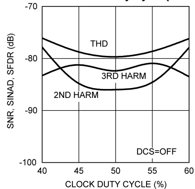
Distortion vs. Clock Duty Cycle (DCS=OFF)
