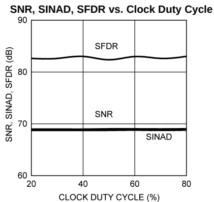
SNR, SINAD, SFDR vs. Clock Duty Cycle (DCS=OFF)
