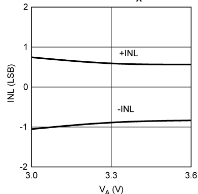
INL vs. V_A
