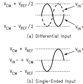
Figure 3. Expected Input Signal Range
