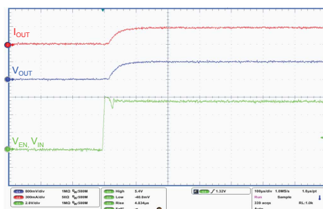
Figure 40. Turn-on time
