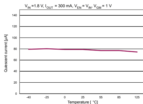
Figure 17. Quiescent current vs. temperature ( I_{OUT} = 300\text{ mA} , normal mode)
