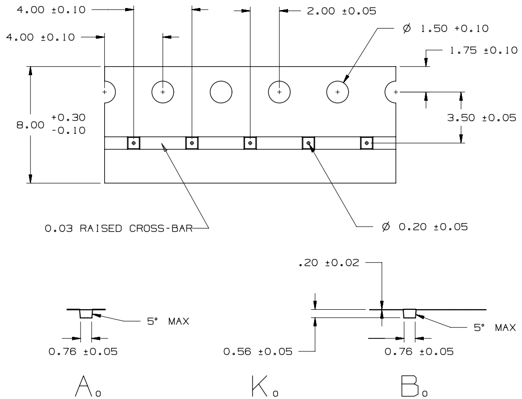
Figure 52. Flip-chip 4 tape
