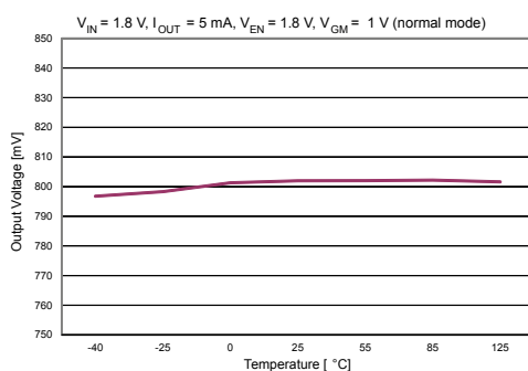
Figure 6. Output voltage vs. temperature ( V_{IN} = 1.8 V , I_{OUT} = 5 mA , normal mode)
