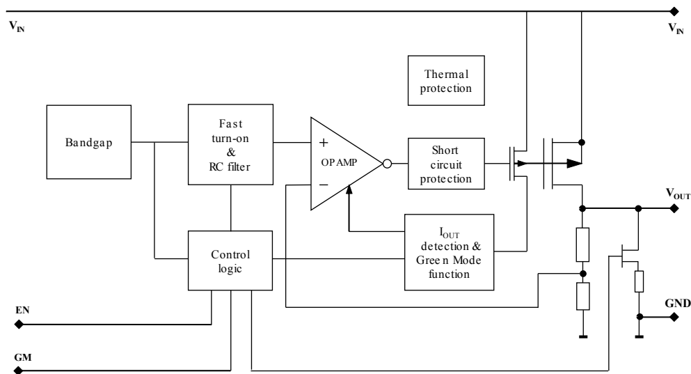
Figure 3. Block diagram (fixed version)
