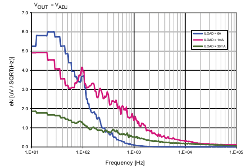
Figure 31. Noise spectrum vs. frequency ( V_{OUT} = V_{ADJ} )
