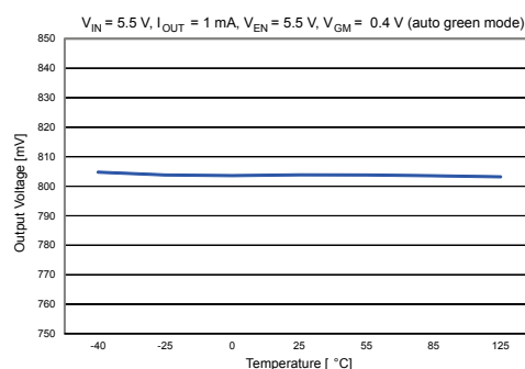
Figure 9. Output voltage vs. temperature ( V_{IN} = 5.5 V , I_{OUT} = 1 mA , auto green mode)
