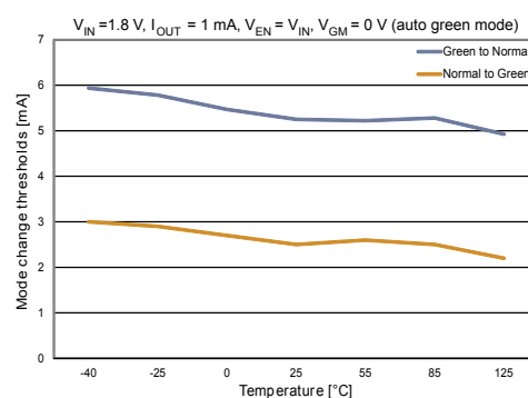
Figure 15. Mode change thresholds vs. temperature
