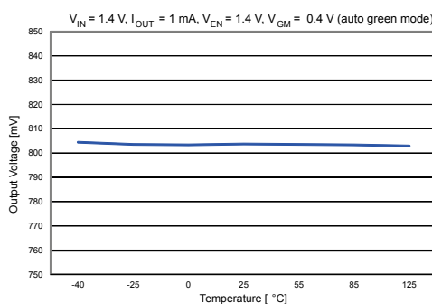
Figure 8. Output voltage vs. temperature ( V_{IN} = 1.4 V , I_{OUT} = 1 mA , auto green mode)
