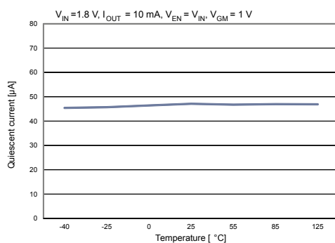
Figure 16. Quiescent current vs. temperature ( I_{OUT} = 10\text{ mA} , normal mode)
