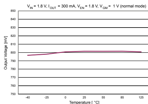
Figure 7. Output voltage vs. temperature ( V_{IN} = 1.8 V , I_{OUT} = 300 mA , normal mode)
