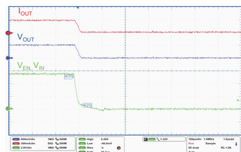
Figure 41. Turn-off time
