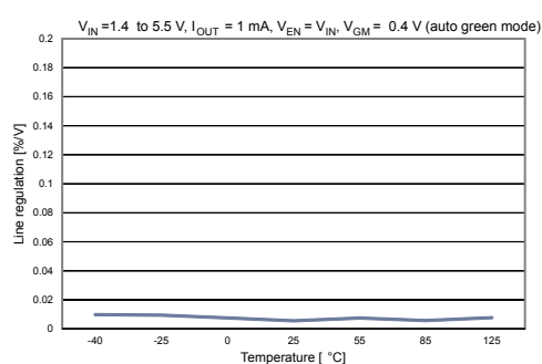
Figure 11. Line regulation vs. temperature (auto green mode)
