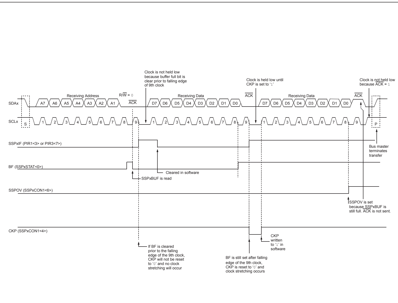
FIGURE 20-15: I 2 C SLAVE MODE TIMING WITH SEN = 1 (RECEPTION, 7-BIT ADDRESS)
