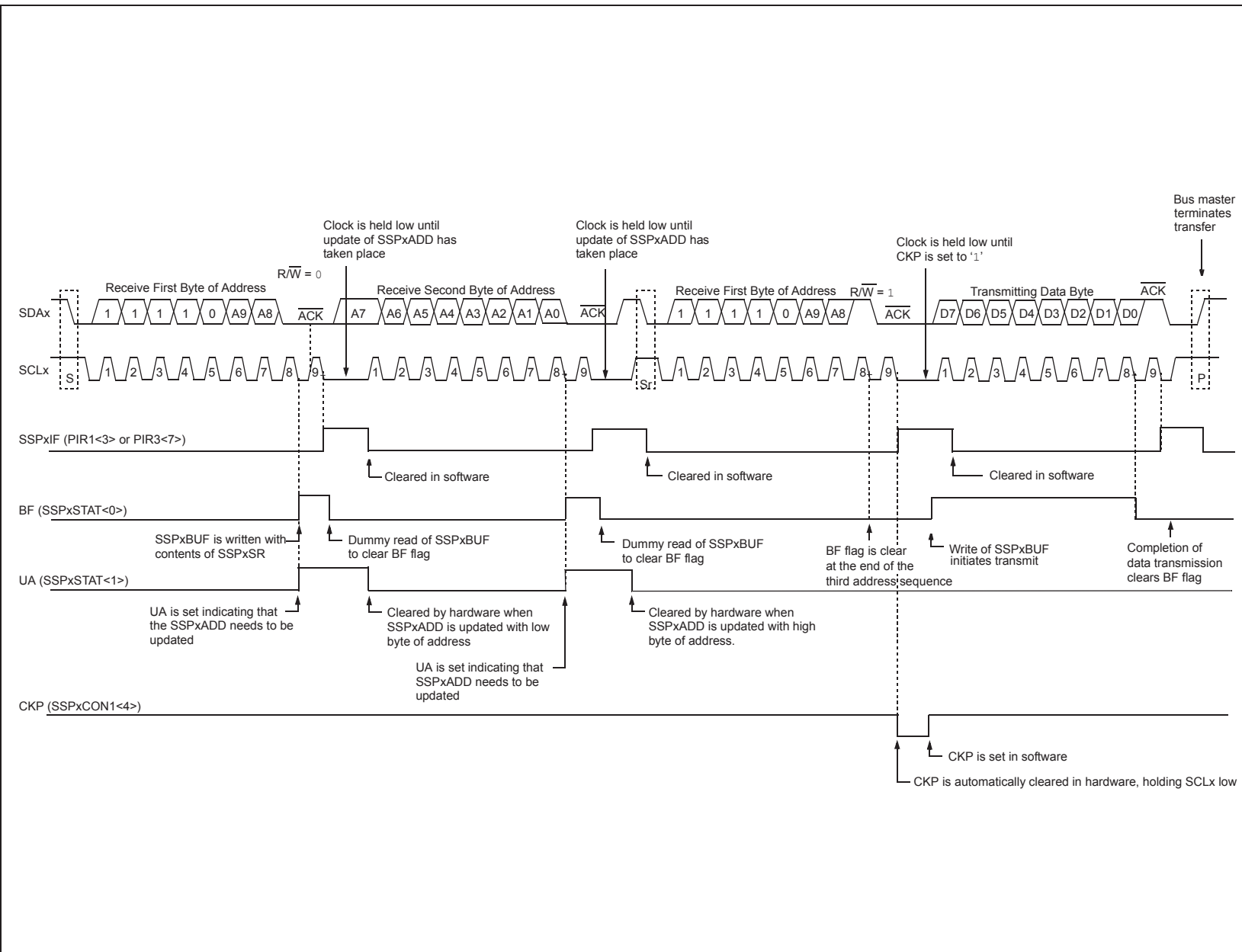
FIGURE 20-13: I 2 C SLAVE MODE TIMING (TRANSMISSION, 10-BIT ADDRESS)
