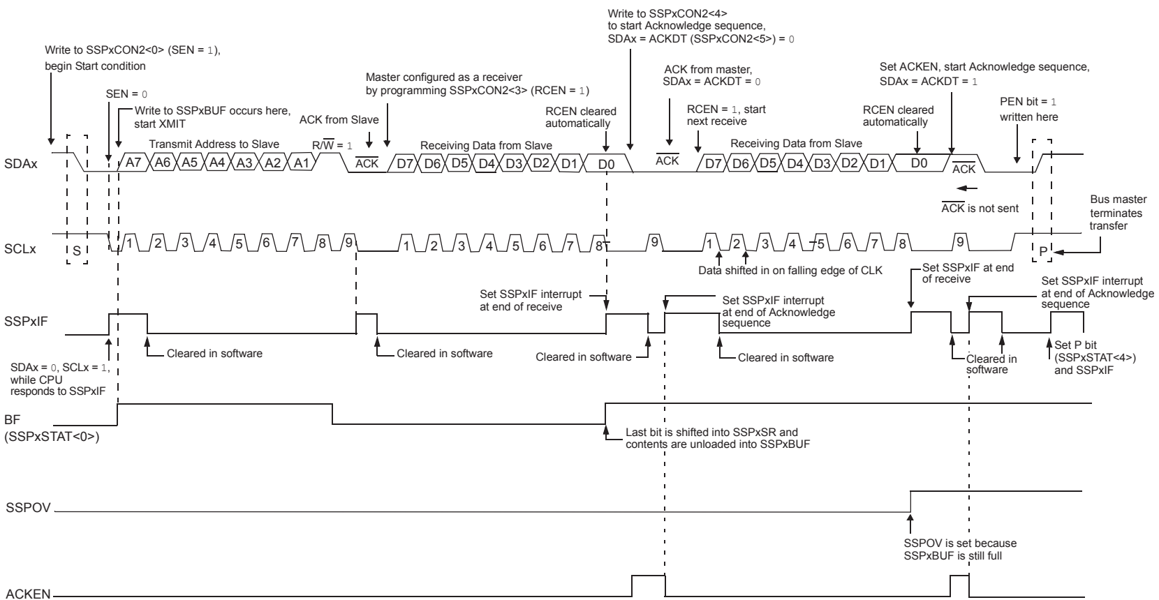
12 C MASTER MODE WAVEFORM (RECEPTION, 7-BIT ADDRESS)
