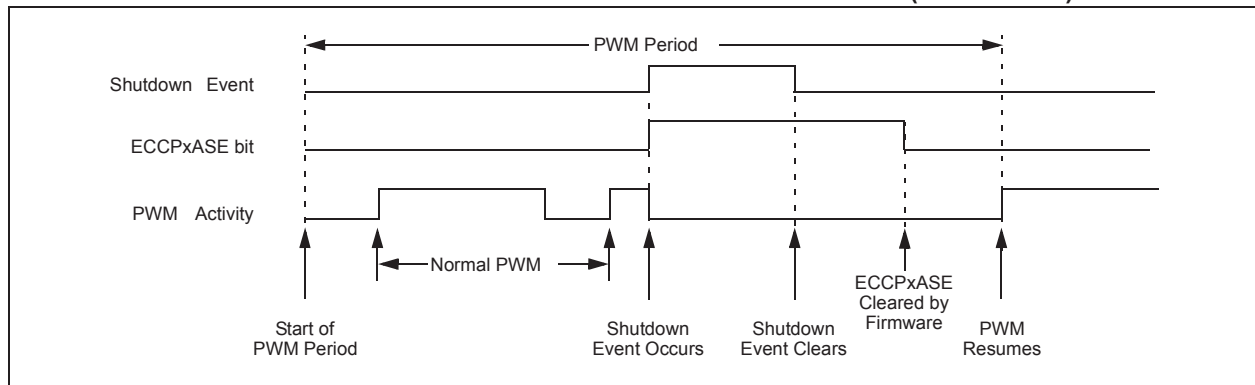
FIGURE 19-12: PWM AUTO-SHUTDOWN WITH FIRMWARE RESTART (PxRSEN = 0)
