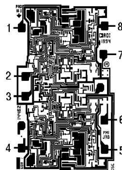
OP284 Die Size 0.065 \times 0.092 Inch, 5,980 Sq. Mils Substrate (Die Backside) Is Connected to V-. Transistor Count, 62.
