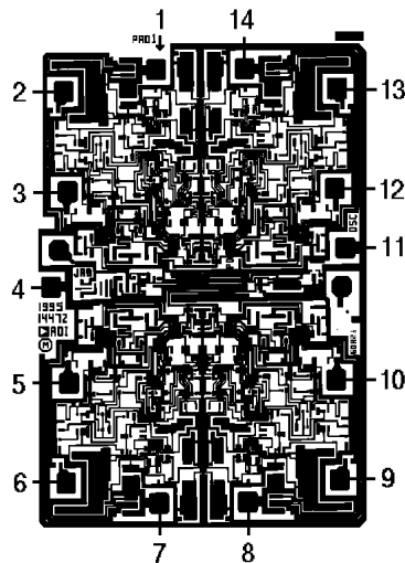
OP484 Die Size 0.080 \times 0.110 Inch, 8,800 Sq. Mils Substrate (Die Backside) Is Connected to V-. Transistor Count, 120.
