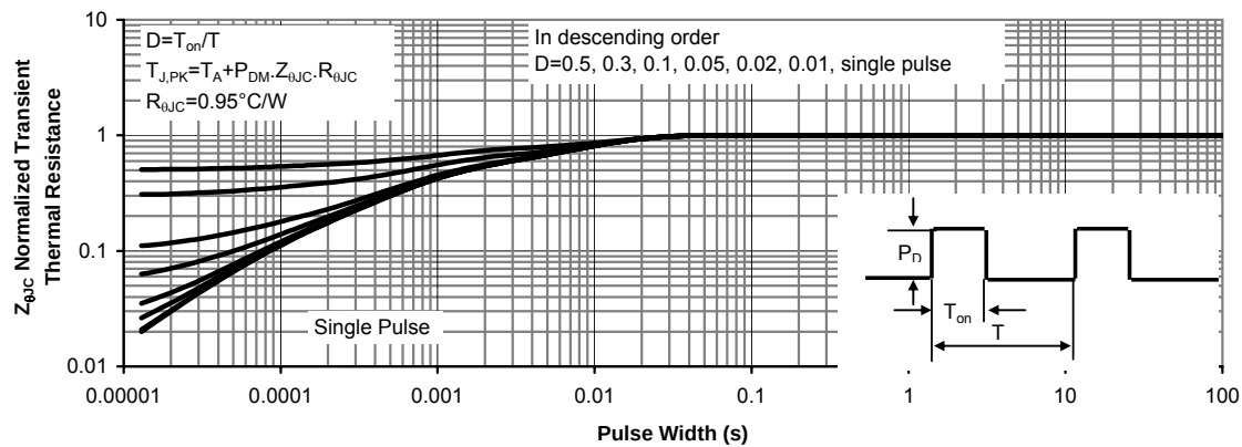
Figure 11: Normalized Maximum Transient Thermal Impedance for AOT5N60 (Note F)
