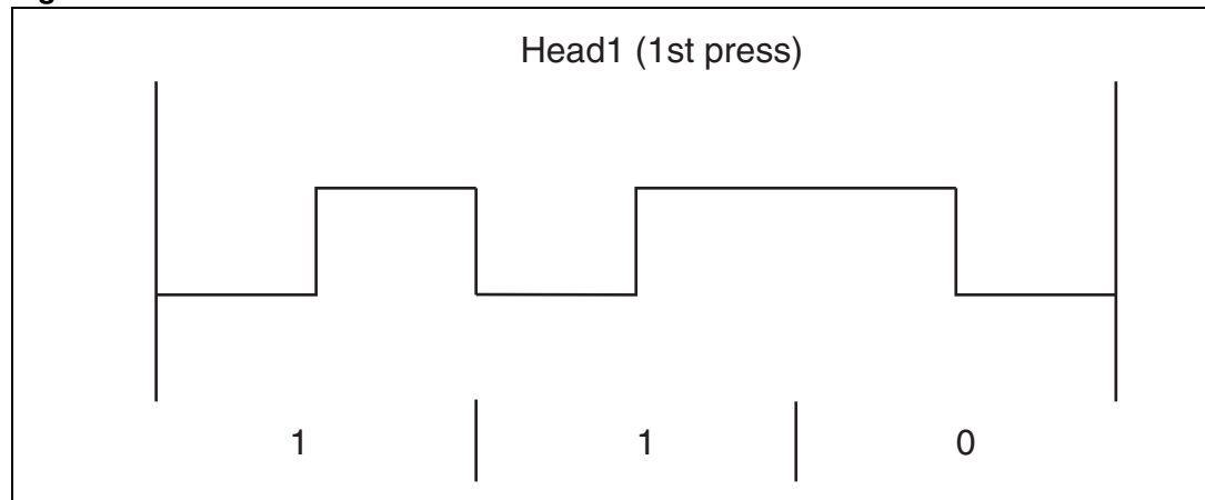
Figure 4. Frame header 1
