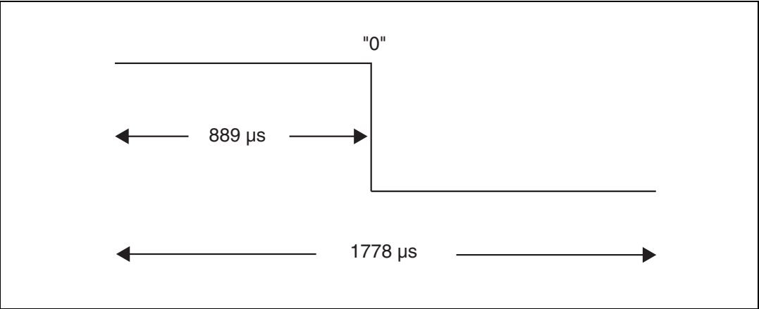
Figure 6. RC5 bit description
