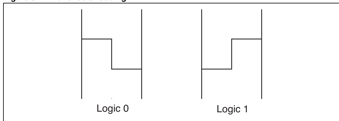
Figure 3. Manchester coding
