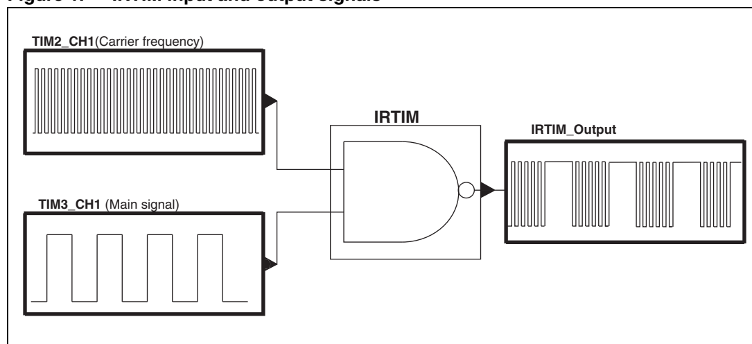
Figure 1. IRTIM input and output signals
