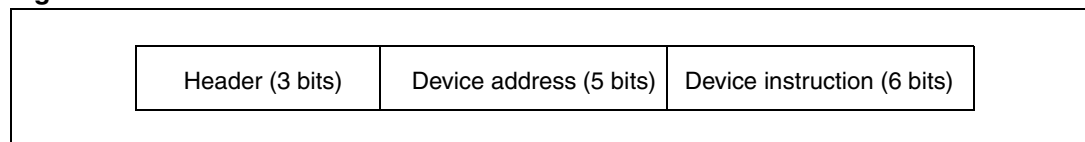
Figure 2. RC5 frame format
