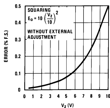
FIGURE 6b. Squaring Mode without External Adjustment
