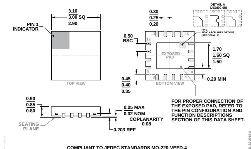
Figure 18. 16-Lead Lead Frame Chip Scale Package [LFCSP] 3 mm × 3 mm Body and 0.85 mm Package Height (CP-16-50) Dimensions shown in millimeters
