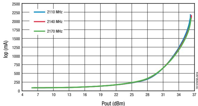
Figure 9. Iop vs Pout Across Frequency
