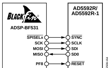
Figure 48. ADSP-BF531 SPI Interface
