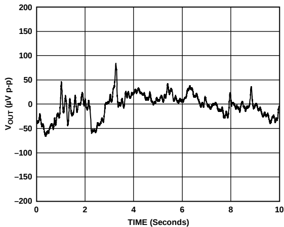
Figure 30. DAC 1/f Noise with Internal Reference
