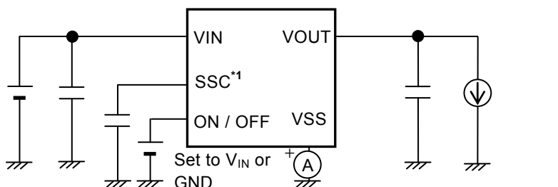
Figure 10 Test Circuit 2
