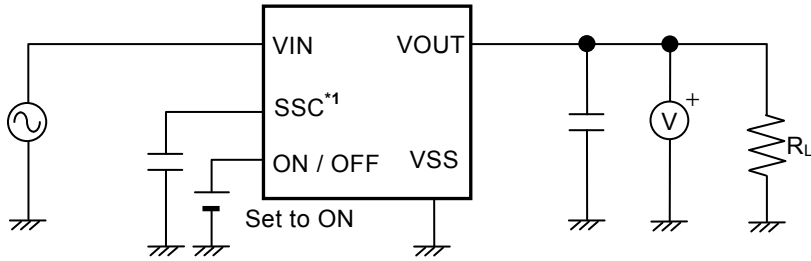
Figure 13 Test Circuit 5
