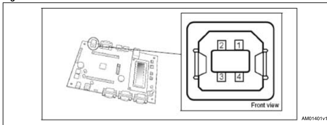
Figure 5. USB connector
