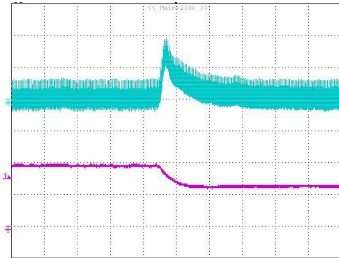
Figure 8: Output voltage response to step-change in load current (75%-50% of I_o , max; di/dt = 1A/\mu s ). Load cap: 2310uF electrolytic capacitor. Top Trace: Vout (20mV/div, 100us/div), Bottom Trace: I_o (20A/div, 100us/div), Scope measurement should be made using a BNC cable (length shorter than 20 inches). Position the load between 51 mm to 76 mm (2 inches to 3 inches) from the module.
