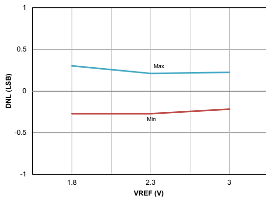
Figure 39-9. ADC 10-BIT, DNL, Vdd = 3.0V, TAD = 1μS, Min and Max values at 125C + 3σ
