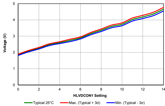
Figure 39-60. LVD Comparator Output High Trip Points
