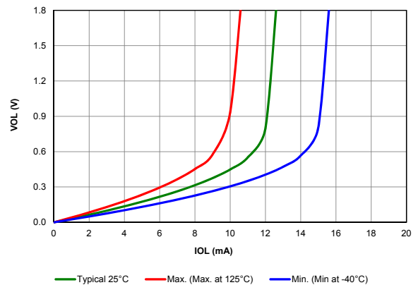
Figure 39-81. VOL vs. IOL OVER TEMPERATURE, VDD = 1.8V
