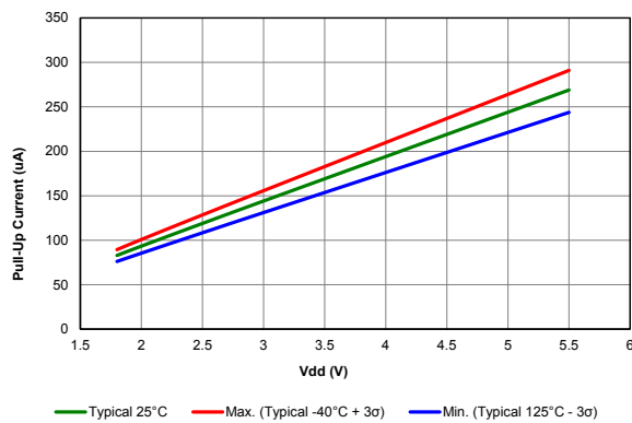
Figure 39-84. Weak Pull Up Current
