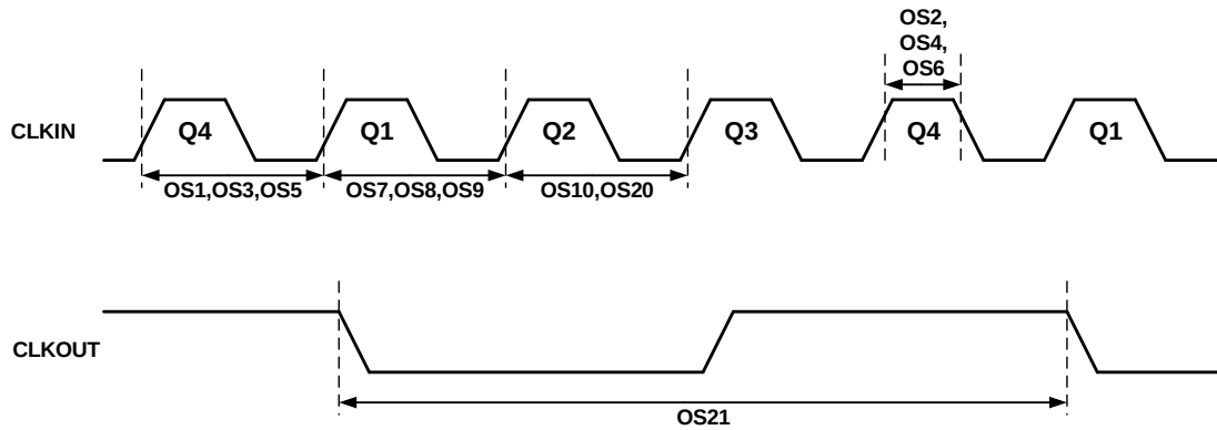
Figure 38-4. Clock Timing
