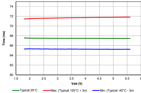
Figure 39-66. PWRT PERIOD vs. V_{DD}
