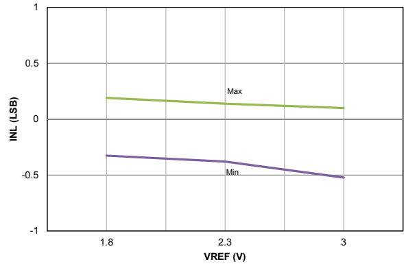
Figure 39-10. ADC 10-BIT, INL, Vdd = 3.0V, TAD = 1μS, Min and Max values at 125C + 3σ
