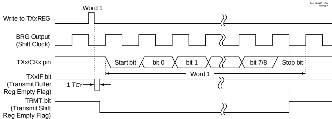
Figure 27-3. Asynchronous Transmission
