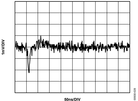
Figure 26. DAC-to-DAC Crosstalk
