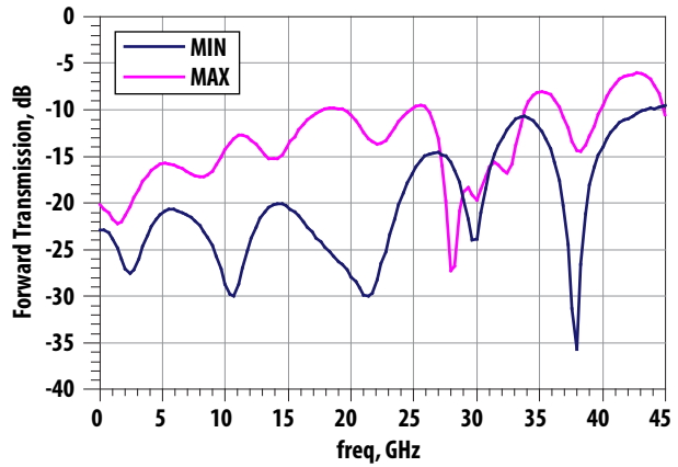
Figure 10b. S22 vs Frequency
