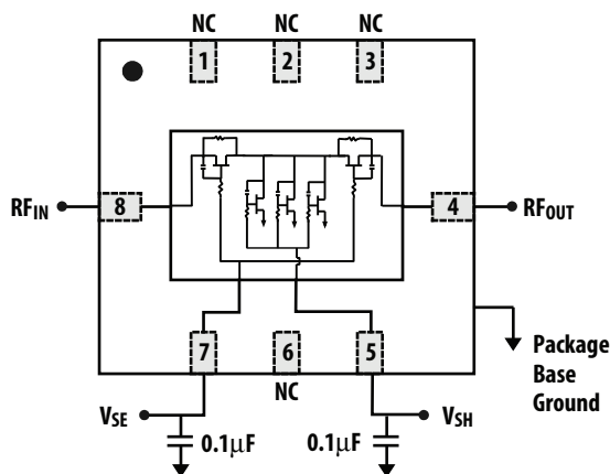
Figure 17. AMMP-6640 Schematic
