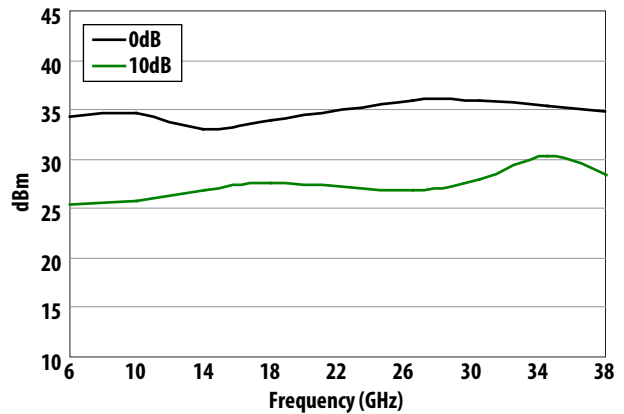
Figure 12. IIP3 vs Attenuation Input Power = 0dBm
