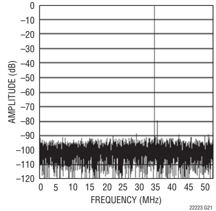
LTC2222: 8192 Point FFT, f_{IN} = 140\text{MHz} , -1\text{dB} , 1V Range
