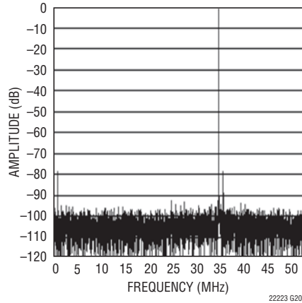
LTC2222: 8192 Point FFT, f_{IN} = 140\text{MHz} , -1\text{dB} , 2V Range
