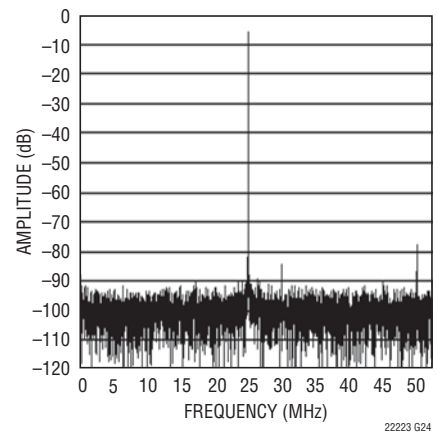
LTC2222: 8192 Point FFT, f_{IN} = 500\text{MHz} , -6\text{dB} , 1V Range
