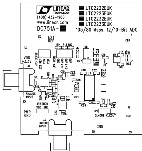
Silkscreen Top
