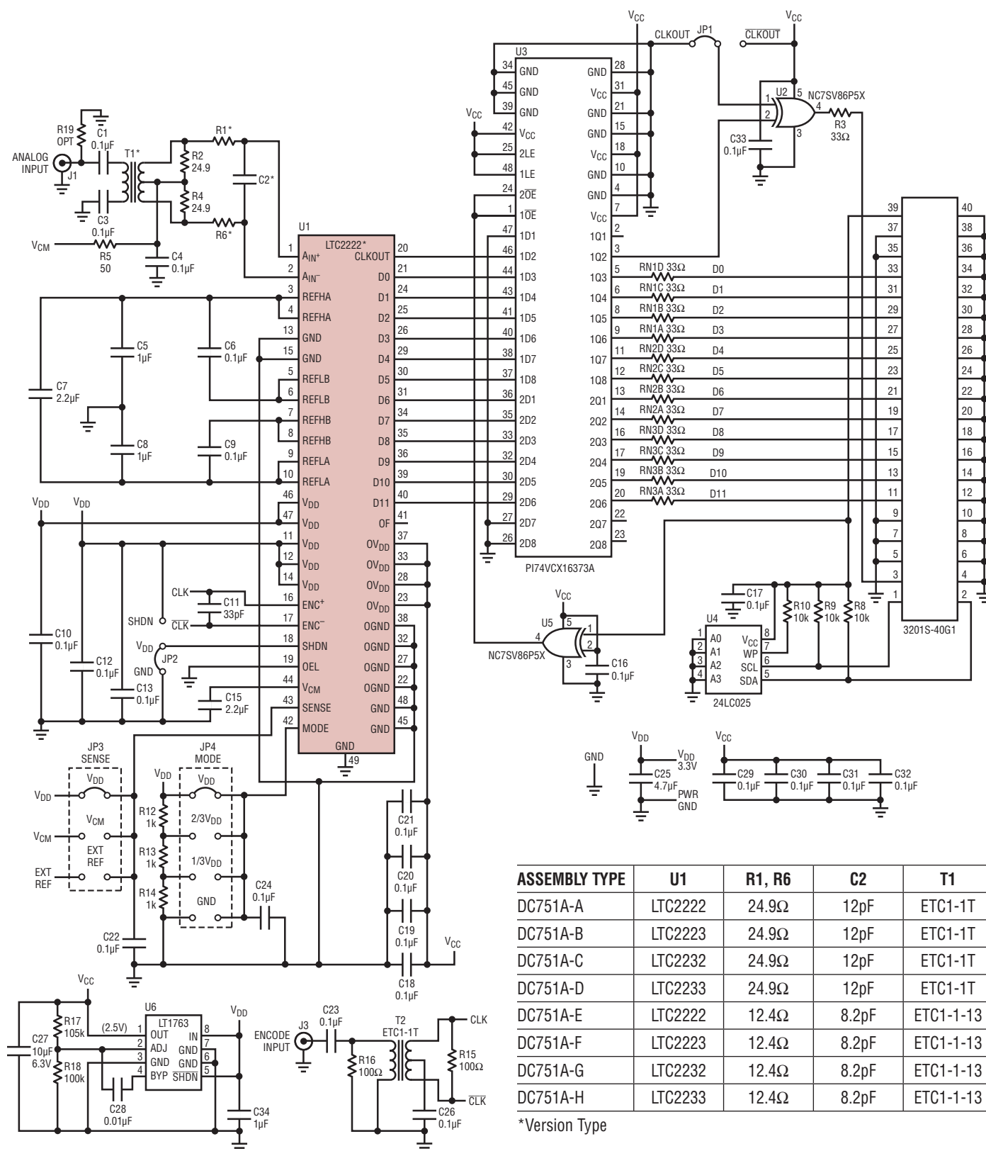
Evaluation Circuit Schematic of the LTC2222
