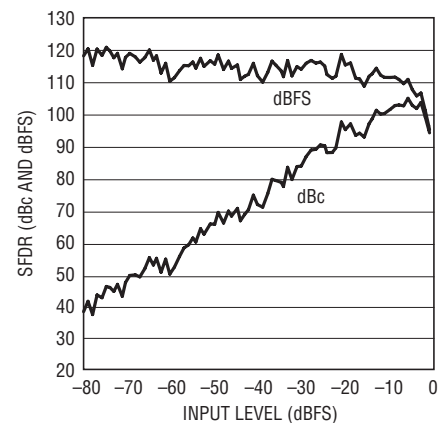
LTC2160: SFDR vs Input Level, f_{IN} = 70\text{MHz} , 25\text{Mps} , 2\text{V} Range
