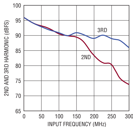
LTC2160: 2nd, 3rd Harmonic vs Input Frequency, -1\text{dBFS} , 25\text{Mps} , 1\text{V} Range
