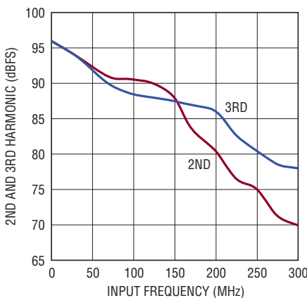
LTC2160: 2nd, 3rd Harmonic vs Input Frequency, -1\text{dBFS} , 25\text{Mps} , 2\text{V} Range
