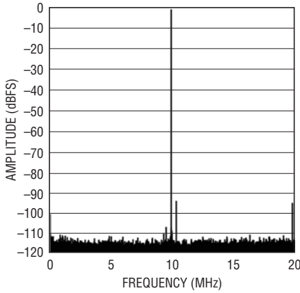
LTC2161: 64k Point FFT, f_{IN} = 30\text{MHz} , -1\text{dBFS} , 40Mps
