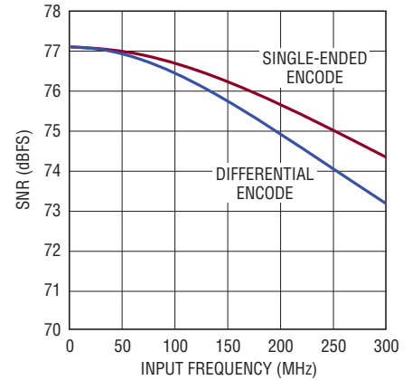
LTC2160: SNR vs Input Frequency, -1\text{dBFS} , 25\text{Mps} , 2\text{V} Range
