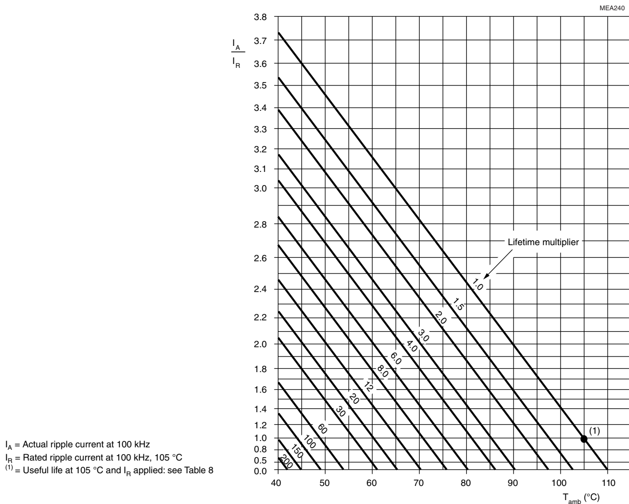
Fig. 15 - Multiplier of useful life as a function of ambient temperature and ripple current load
