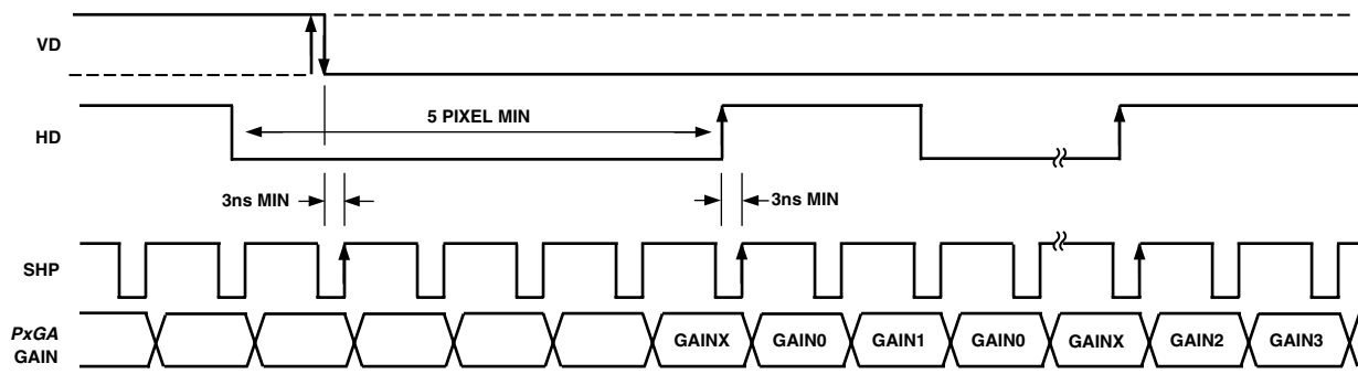
Figure 11. PxGA Mode 2 (Interlace) Detailed Timing
