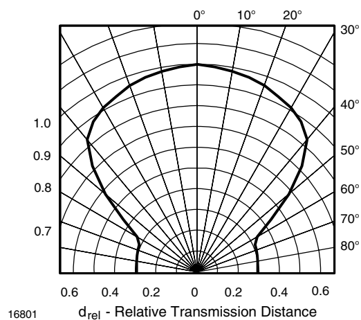
Fig. 10 - Horizontal Directivity
