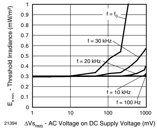
Fig. 6 - Sensitivity vs. Supply Voltage Disturbances
