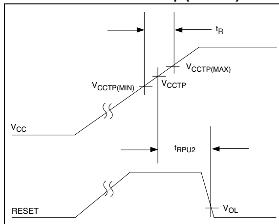
FIGURE 3-3: Timing Diagram – Power Up (TC1278)
