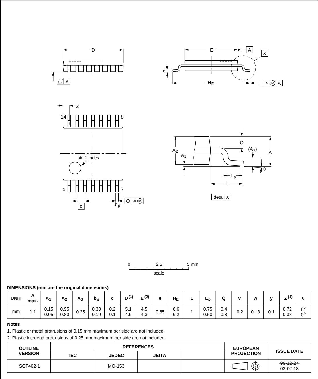
TSSOP14: plastic thin shrink small outline package; 14 leads; body width 4.4 mm SOT402-1
