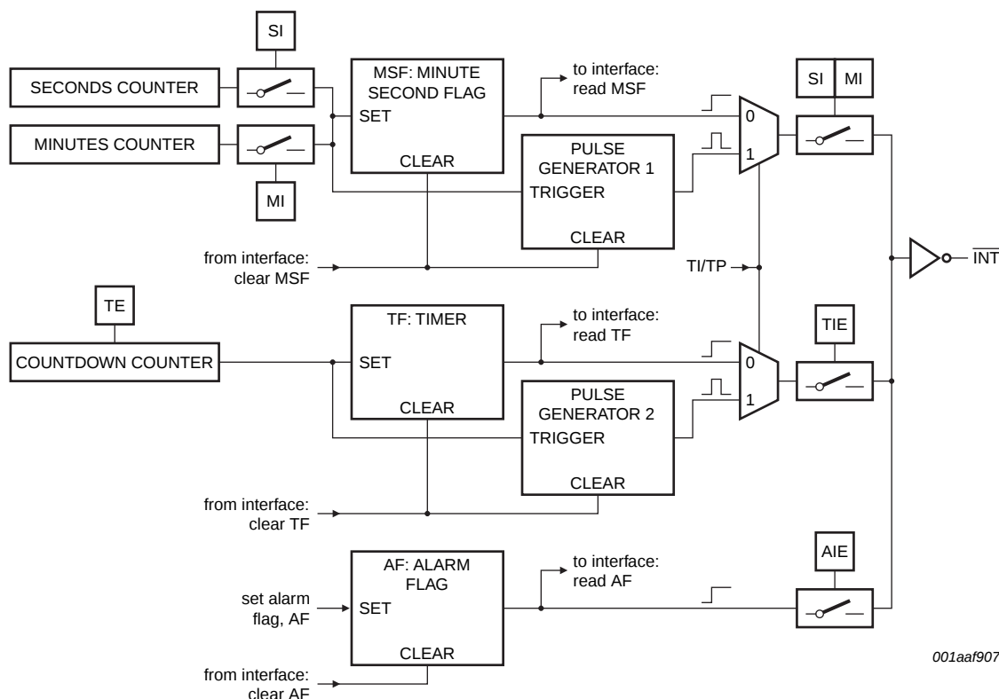
Fig 12. Interrupt scheme
