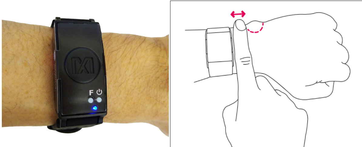
Figure 4. PPG measurement.
