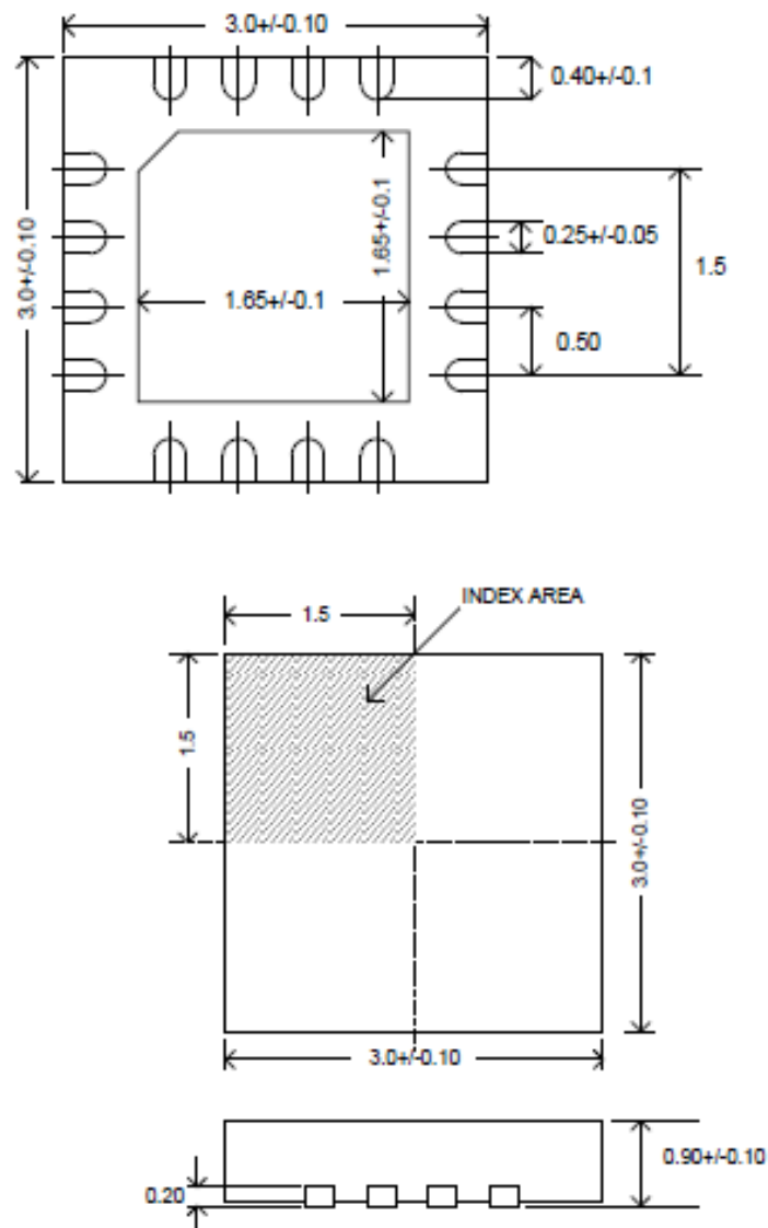
Figure 5.1 ZSPM4011B Package Drawing
