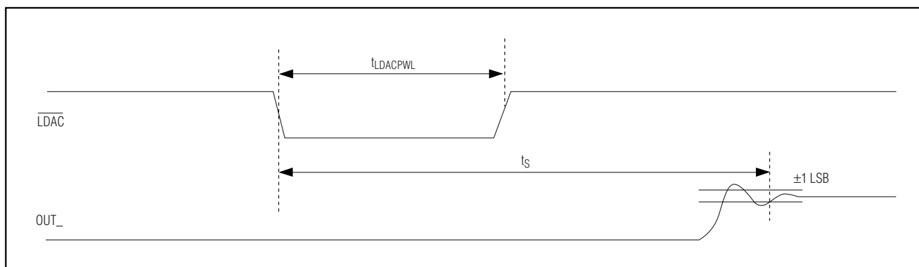
Figure 14. LDAC Functionality
