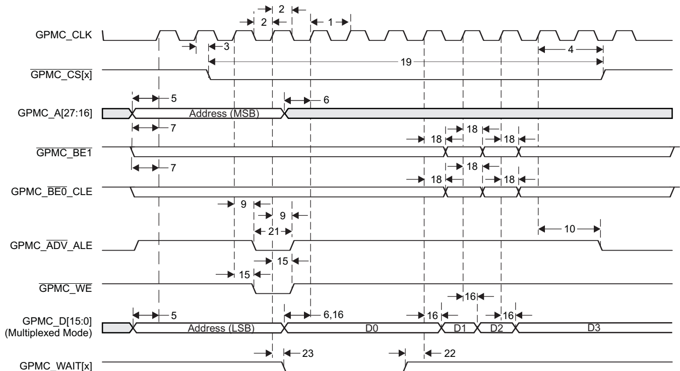
Figure 8-15. GPMC Non-Multiplexed NOR Flash - Synchronous Burst Write (GPMCCLKDIVIDER = 0)
