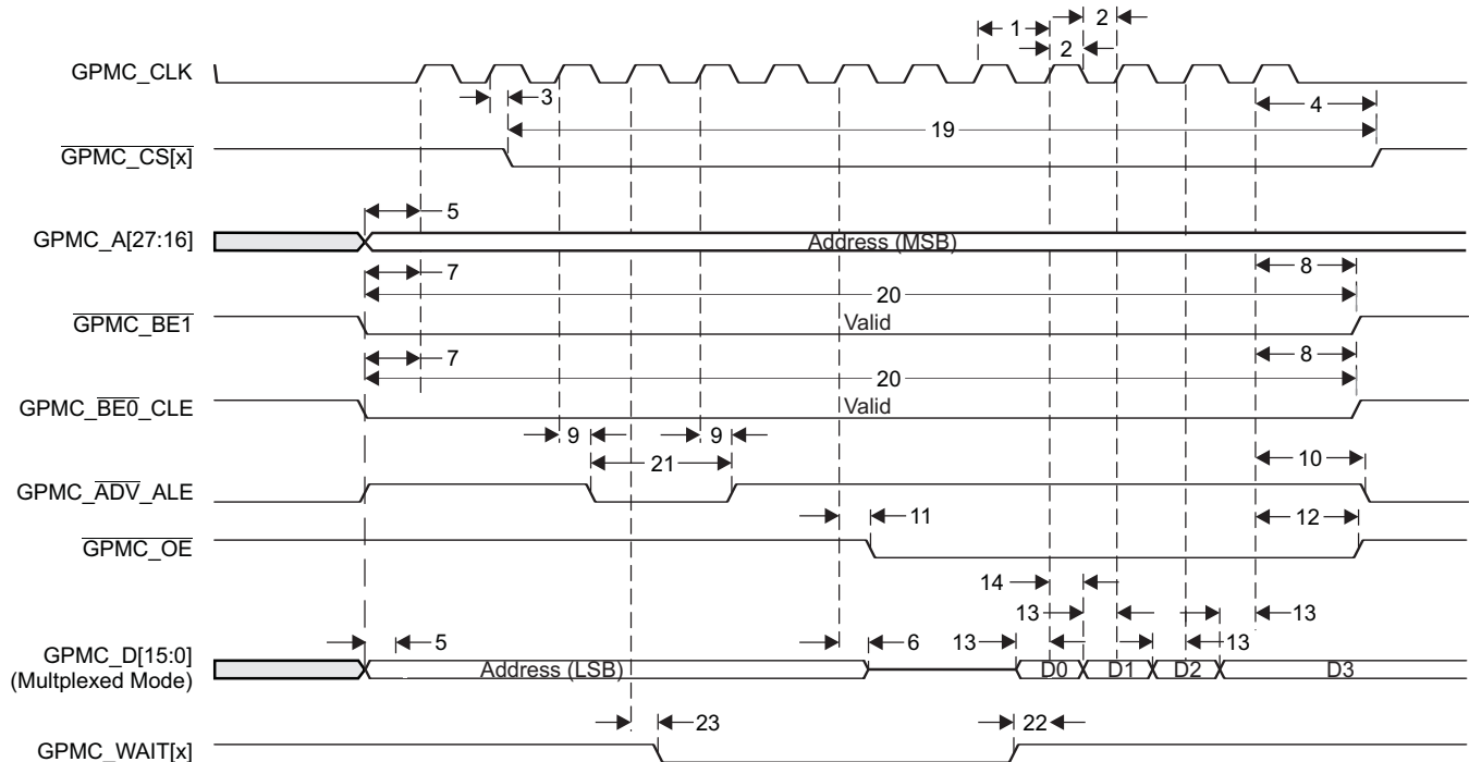
Figure 8-14. GPMC Multiplexed NOR Flash - 14x16-bit Synchronous Burst Read (GPMCCLKDIVIDER = 0)
