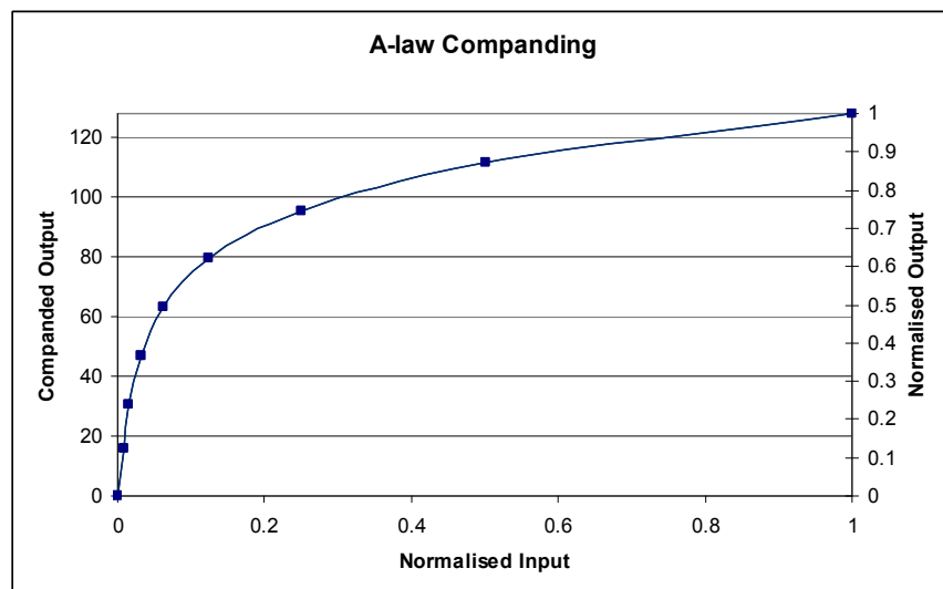
Figure 51 A-Law Companding
