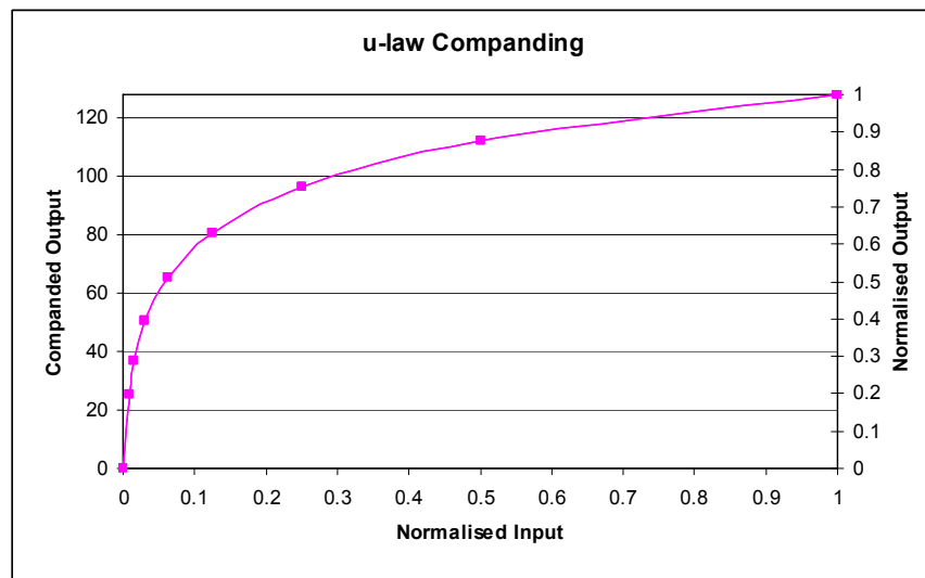
Figure 50 \mu -Law Companding
