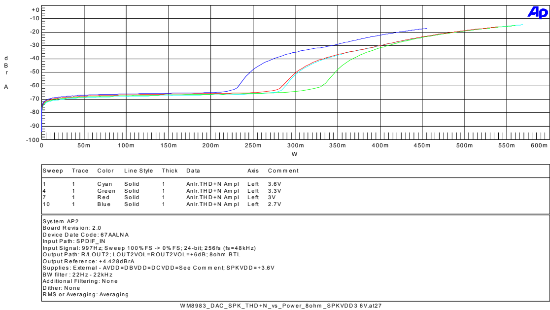
Figure 1 Speaker THD+N vs Output Power (Boost Disabled: SPKVDD=3.6V; SPKBOOST=0; AVDD Range =3.6-2.7V)
