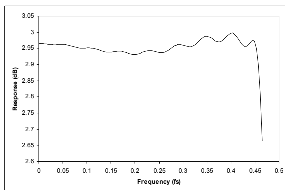
Figure 55 DAC Digital Filter Ripple (128xOSR)
