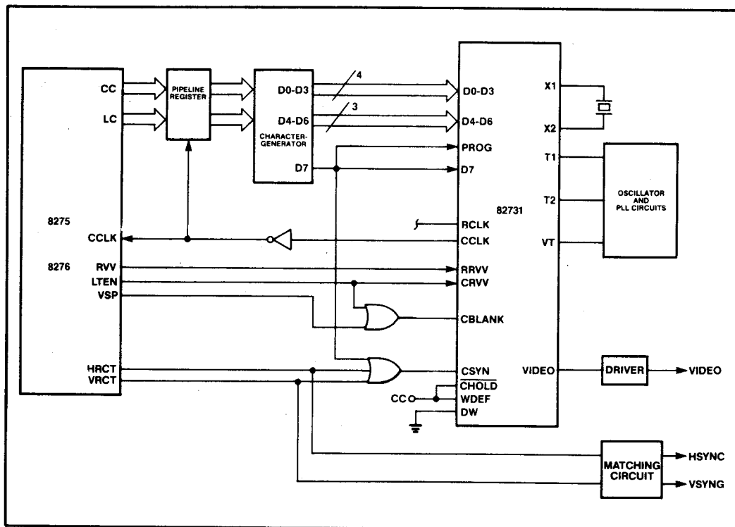
Figure 23. Example Interface to 8275
