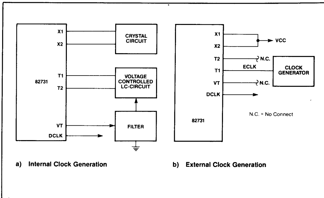
Figure 4. Clock Generation
