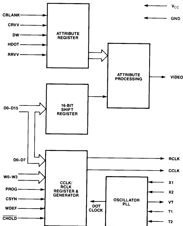
Figure 1. 82731 Block Diagram
