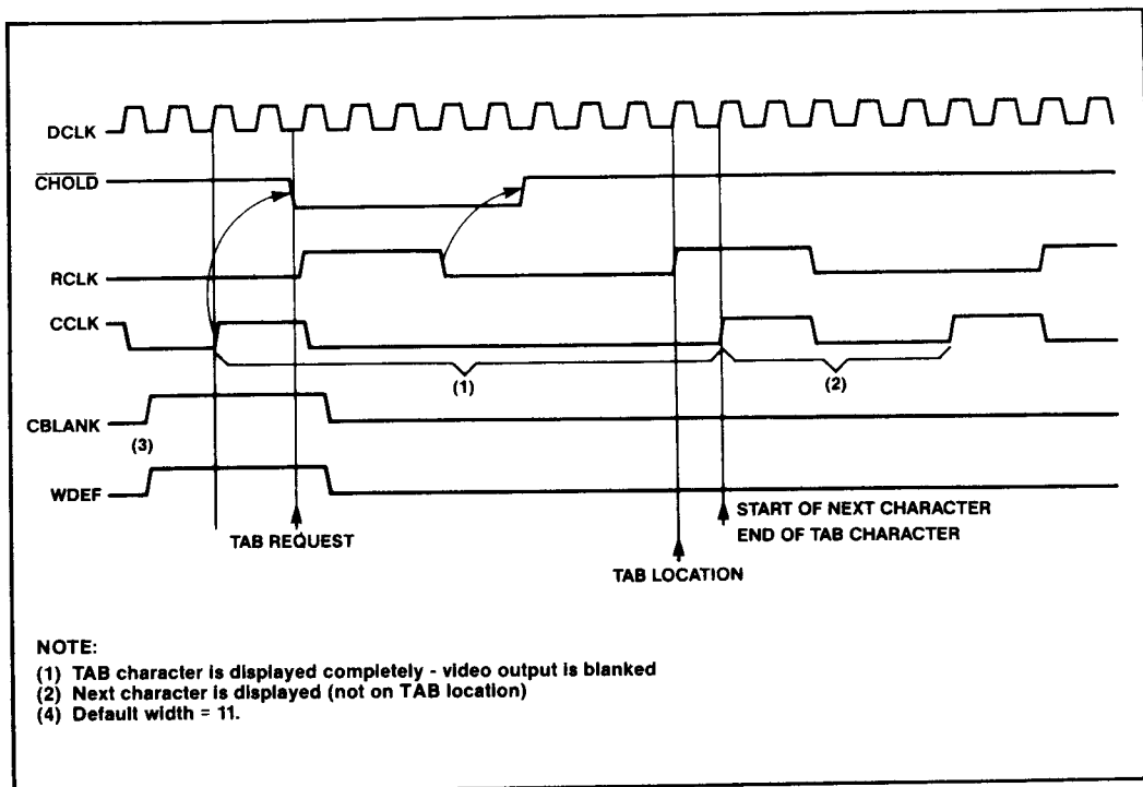
Figure 13. Function of CHOLD with CHOLD Width Less than Character Width (Case 3)
