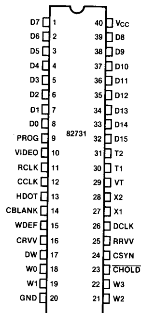
Figure 2. 82731 Pin Configuration
