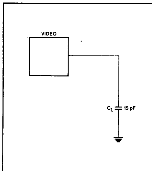
Figure 18. ECL-Level-Output Test
