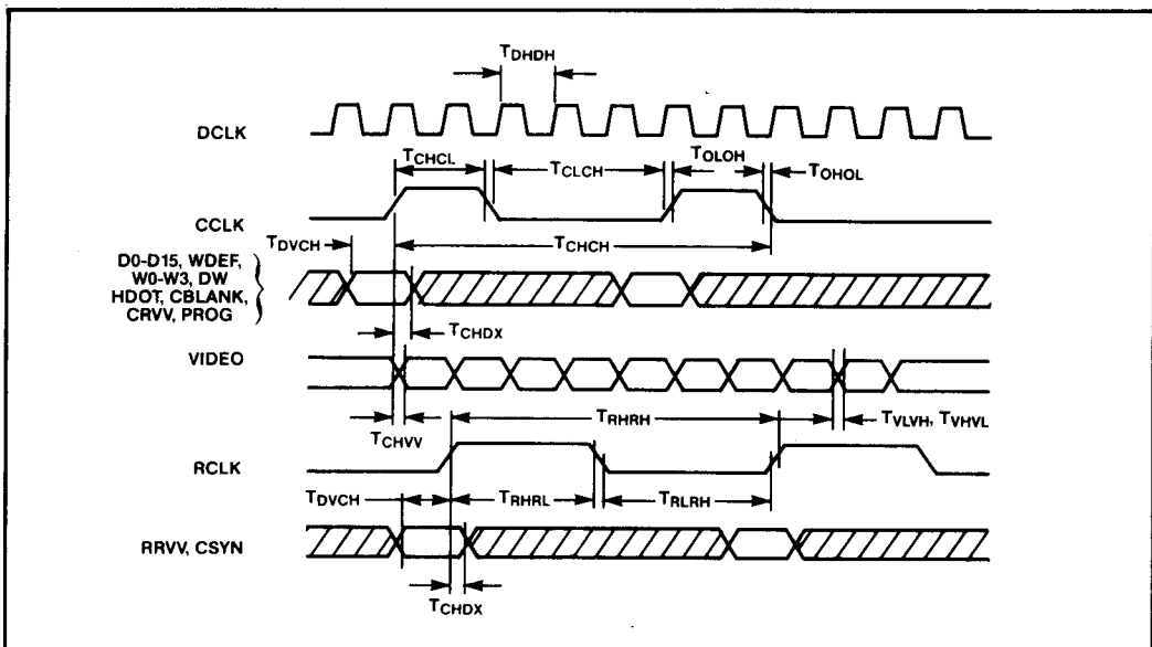
Figure 21. Basic Timing
