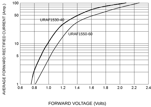
FIG-1 TYPICAL FORWARD CHARACTERISITICS
