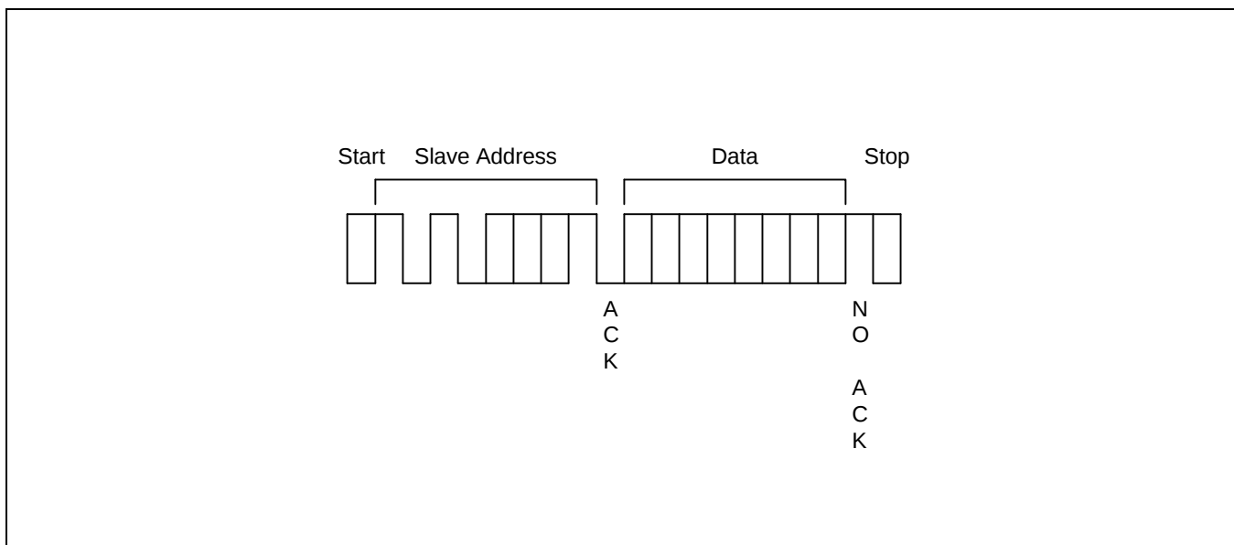
Figure 8-13. Current Address Byte Read Operation
