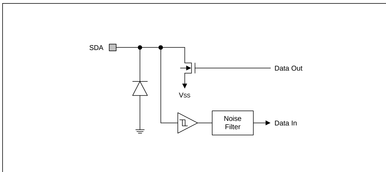
Figure 8-5. Pin Circuit Type 3
