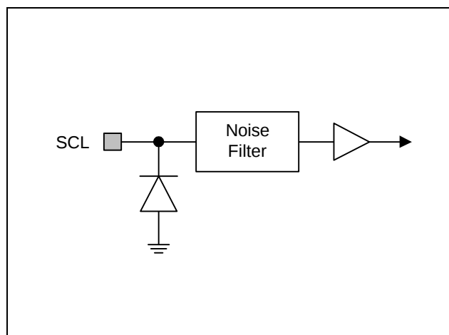
Figure 8-4. Pin Circuit Type 2
