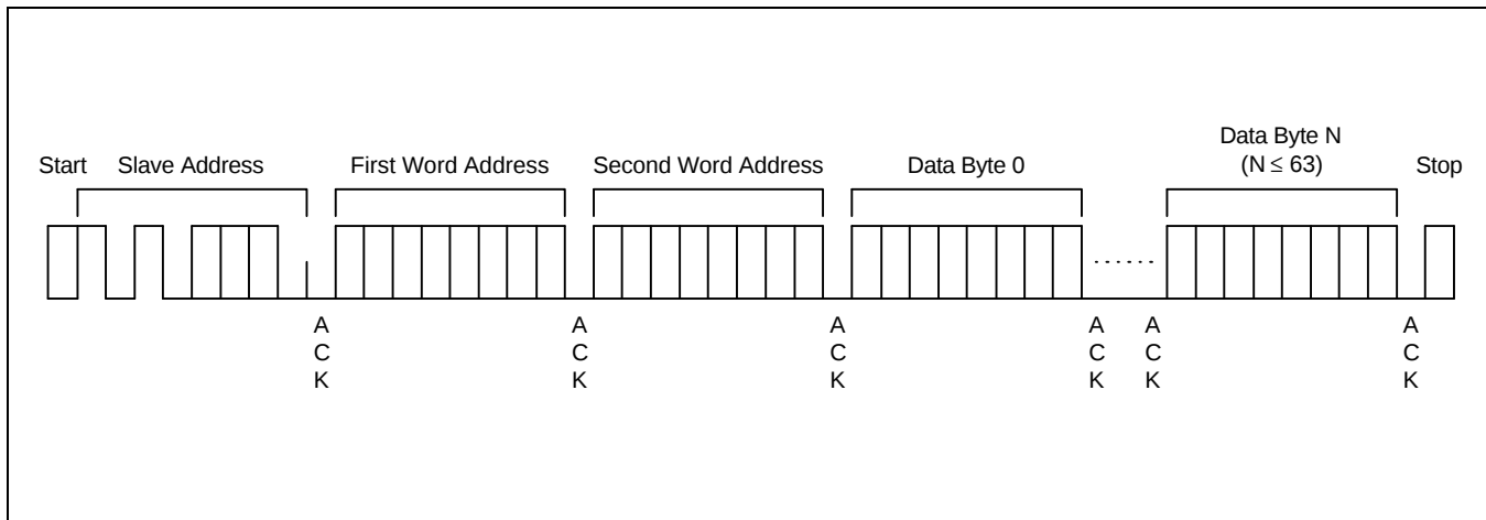
Figure 8-11. Page Write Operation
