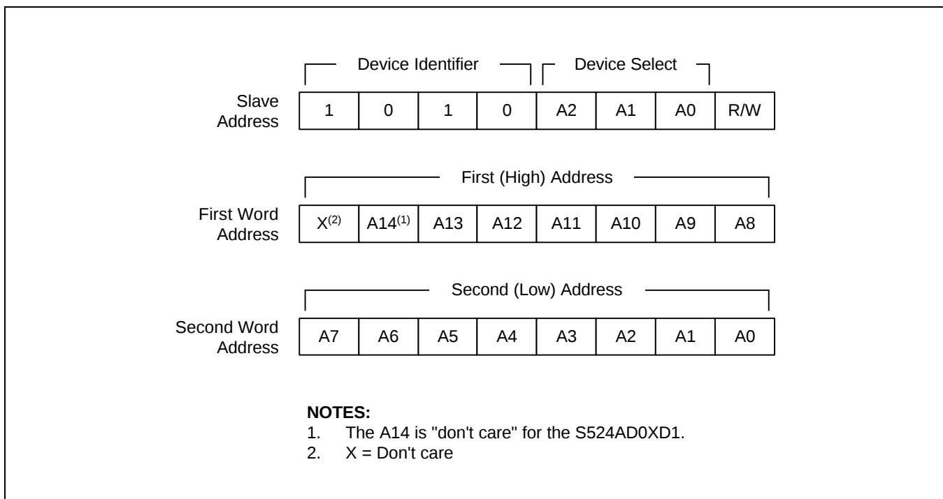
Figure 8-9. Device Address
