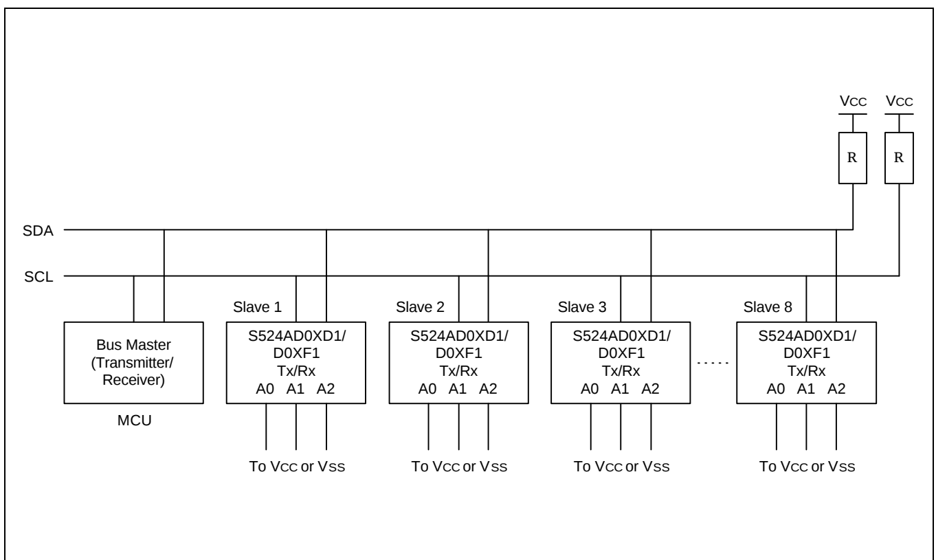
Figure 8-6. Typical Configuration
