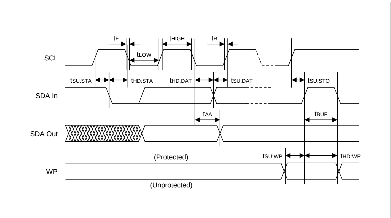
Figure 8-16. Timing Diagram for Bus Operations
