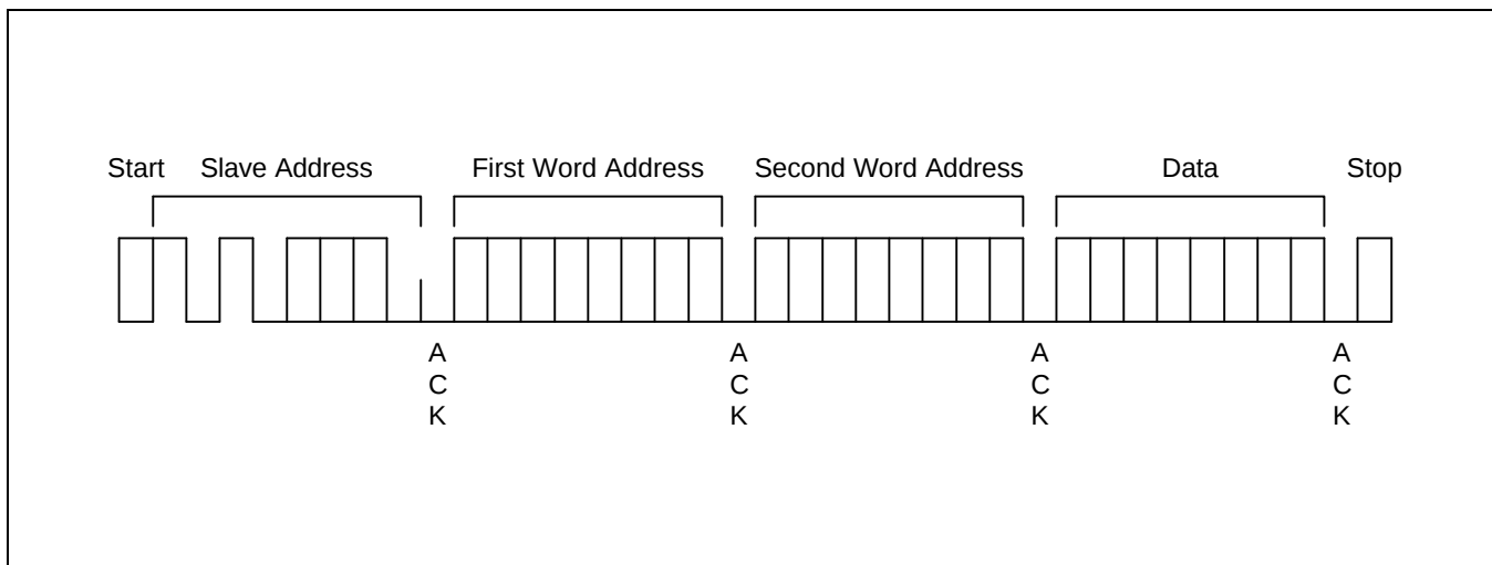
Figure 8-10. Byte Write Operation
