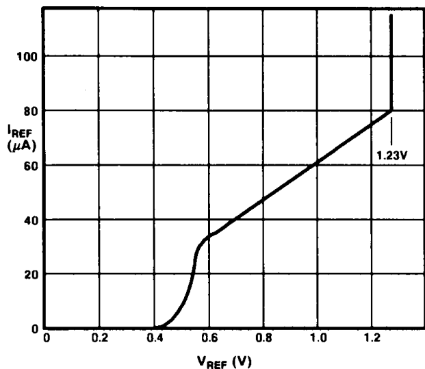
Fig.4 Typical reference characteristic
