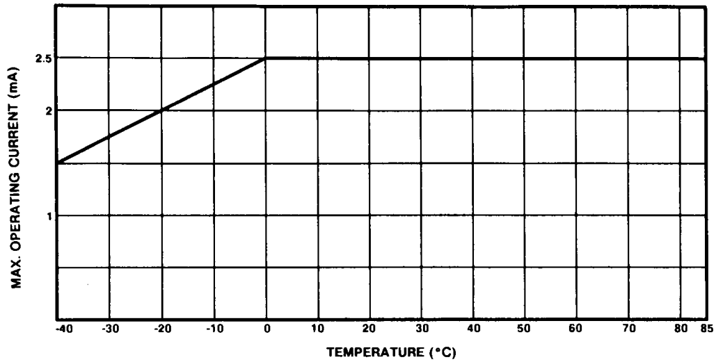
Fig.7 Derating curve
