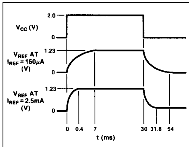
Fig.5 SR12D typical response time (not to scale)
