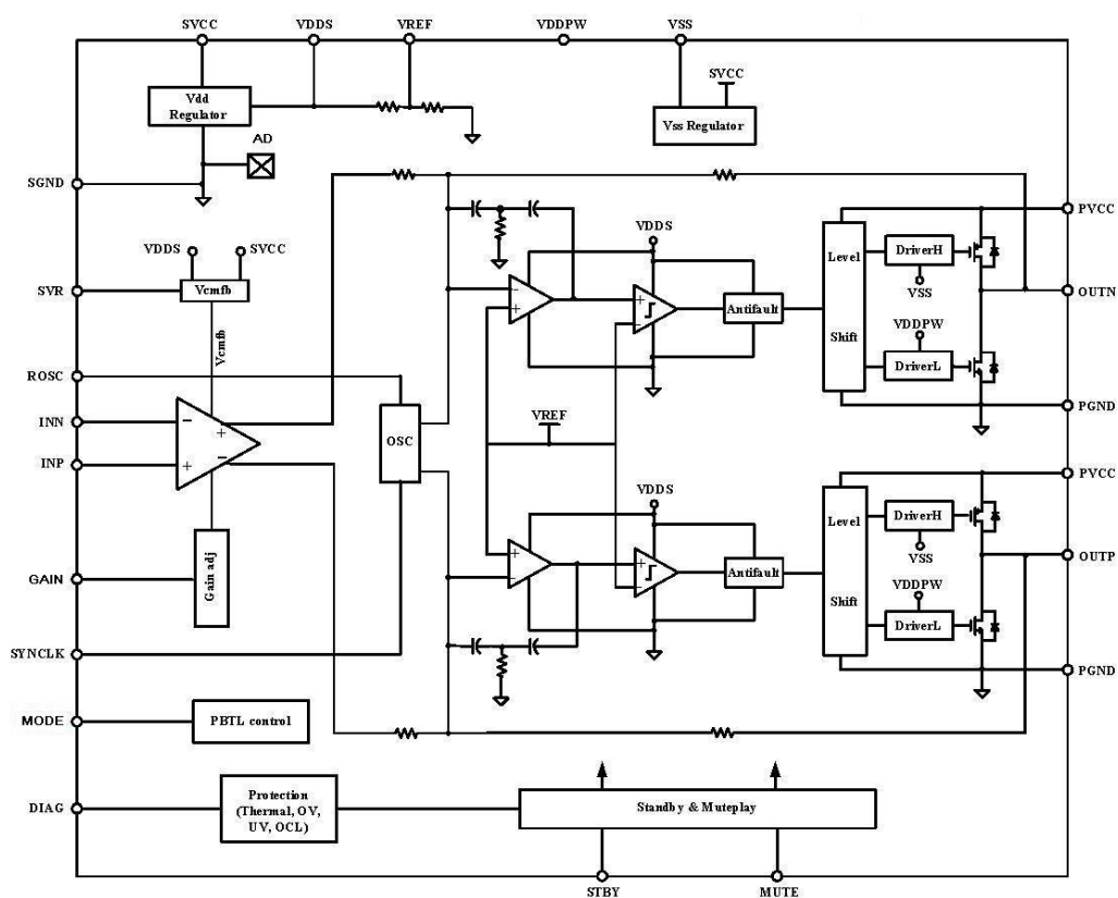
Figure 1. Internal block diagram (showing one channel only)
