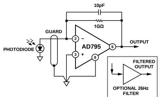
Figure 45. AD795 Used as a Photodiode Preamplifier
