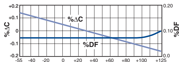
Figure 3. Temperature °C Capacitance & DF vs Temperature - C0G
