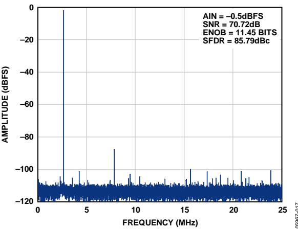
Figure 17. Single-Tone 32k FFT with f_{IN} = 2.3 MHz, AD9222-50
