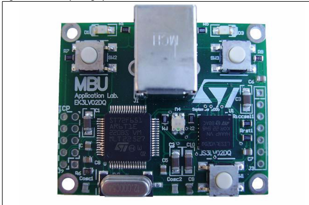
Figure 3. Board photograph
