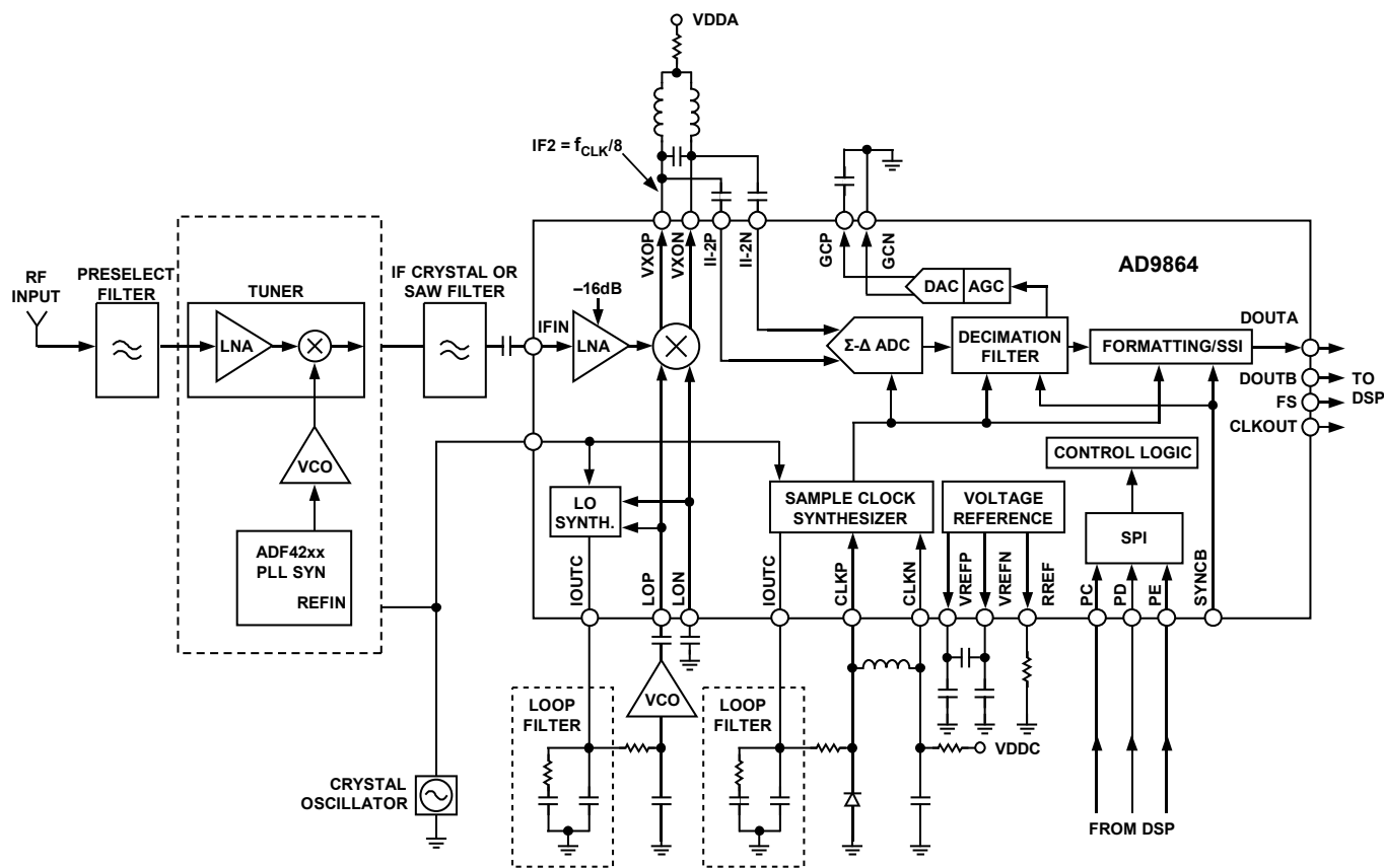
Figure 73. Typical Dual Conversion Superheterodyne Application Using the AD9864
