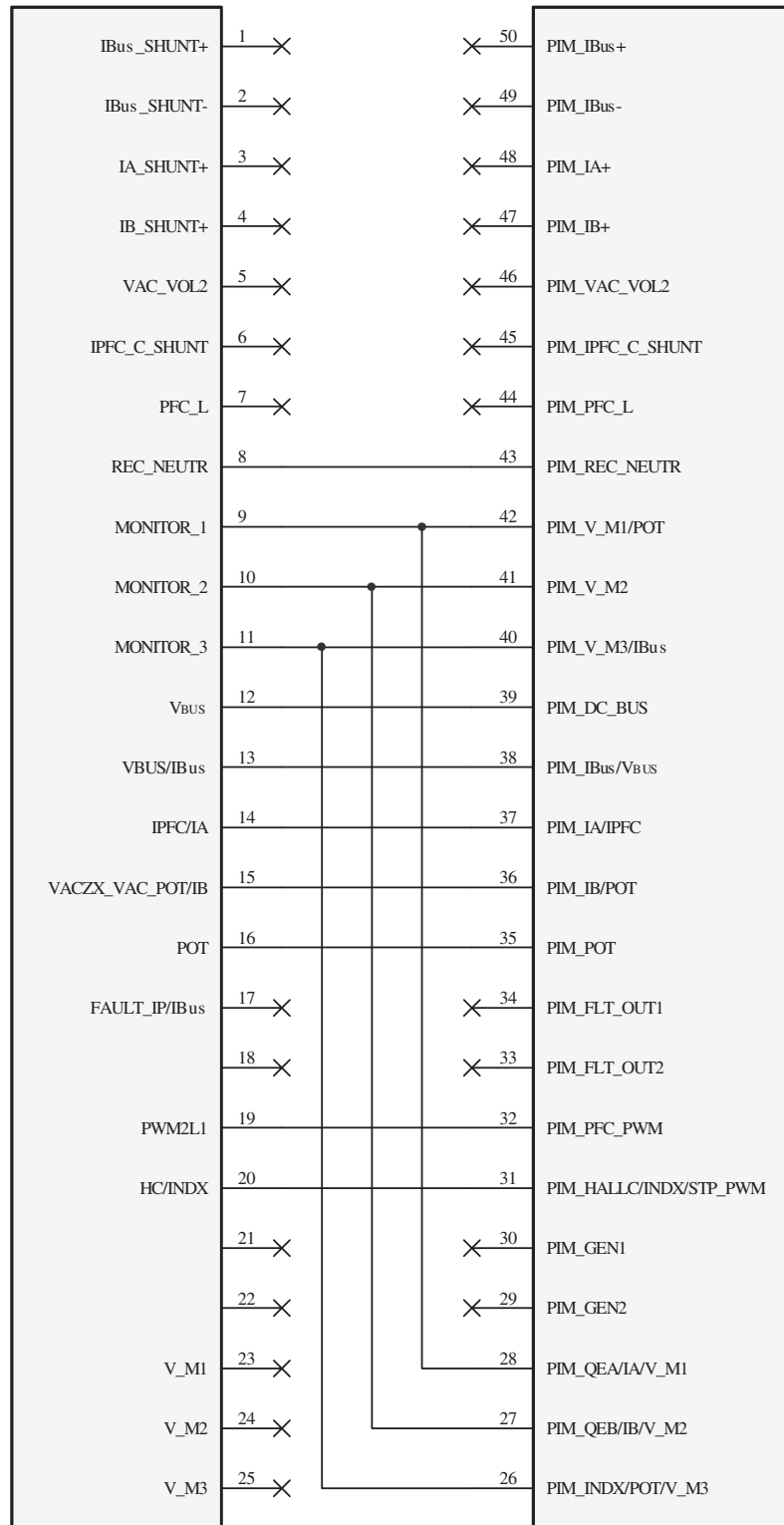
FIGURE A-14: EXTERNAL OP AMP CONFIGURATION MATRIX BOARD SCHEMATIC
