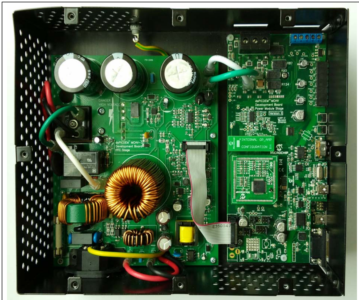
FIGURE 2-1: dsPICDEM™ MCHV-3 DEVELOPMENT BOARD ENCLOSURE VIEW
