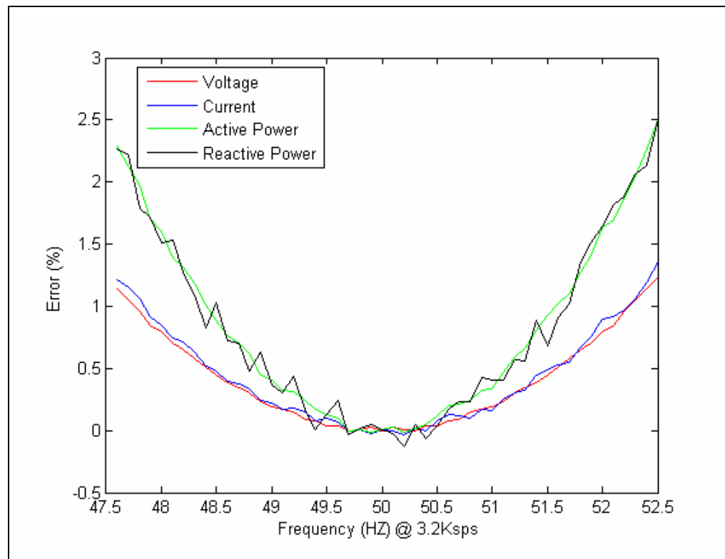
FIGURE C-4: Quasi-sync Algorithm Error Analysis of 3 Iterations.
