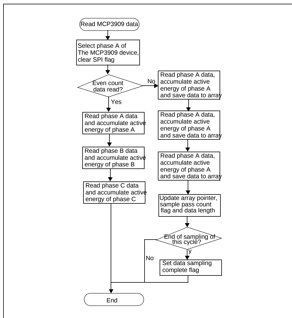
FIGURE 3-5: Flow Chart of Read A/D Data.
