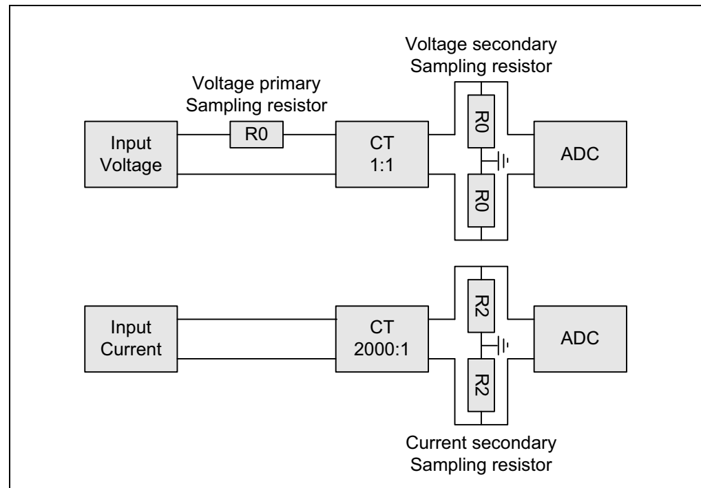
FIGURE C-9: Error Caused By Sampling Circuit And ADC.
