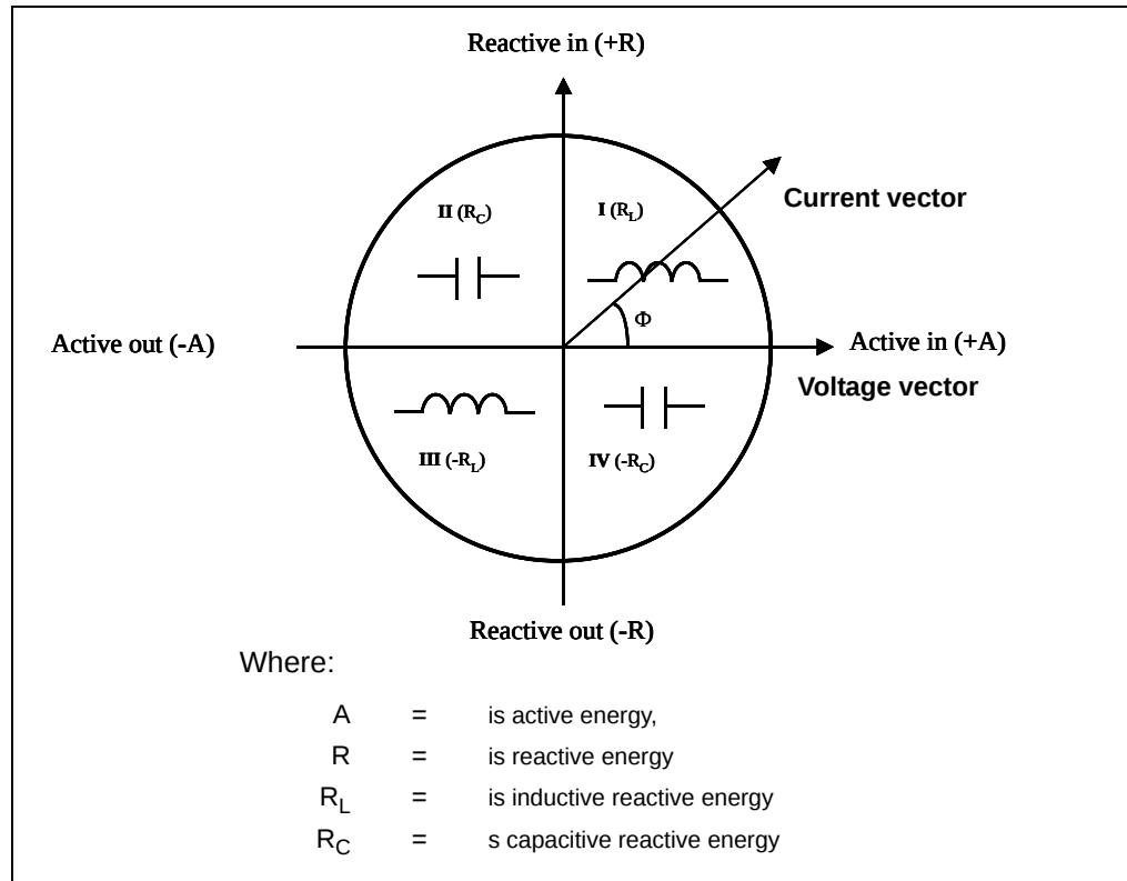
FIGURE C-7: Definition Of 4 Quadrants To Measure Electrical Energy.
