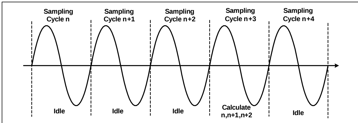
FIGURE 3-3: AC Signal Sampling and Computing.
