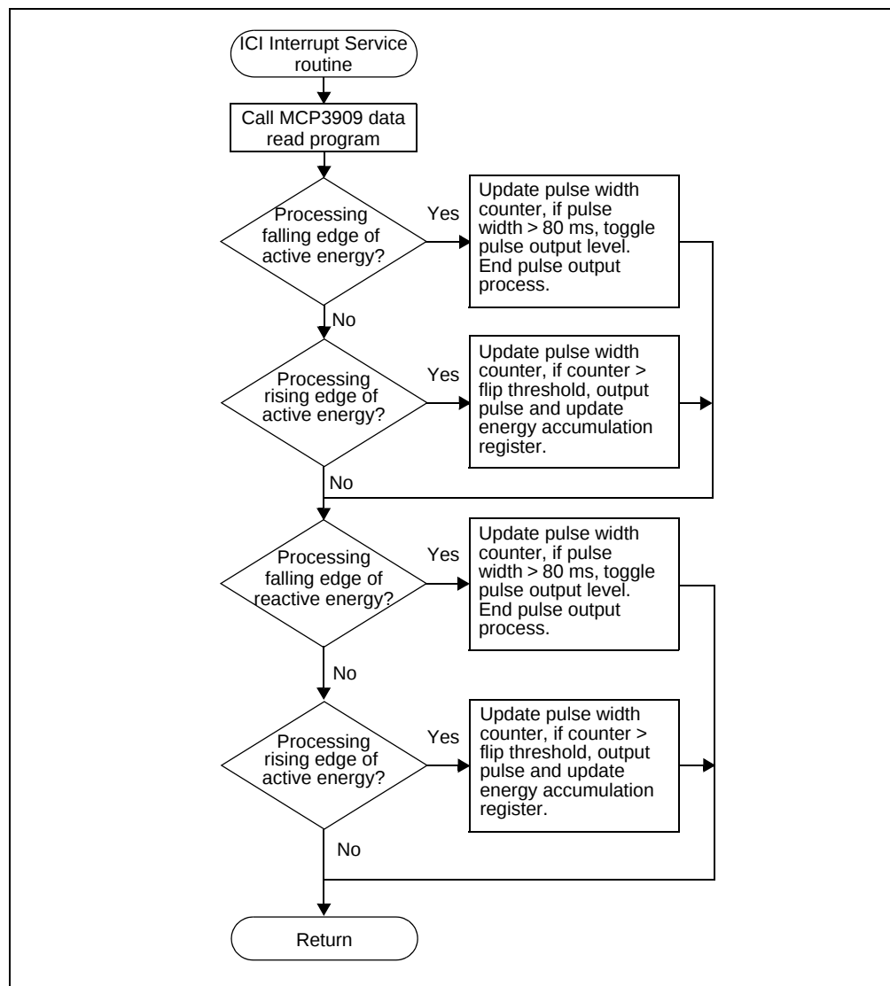
FIGURE 3-4: IC1 Interrupt Service Routine.
