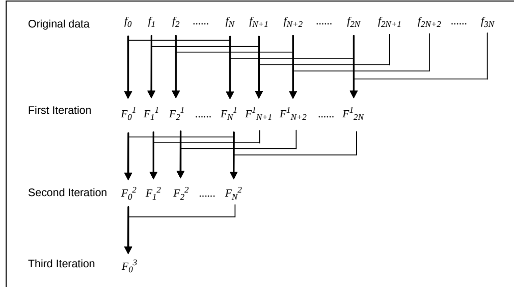
FIGURE C-2: 3-Cycle Iterative Process.
