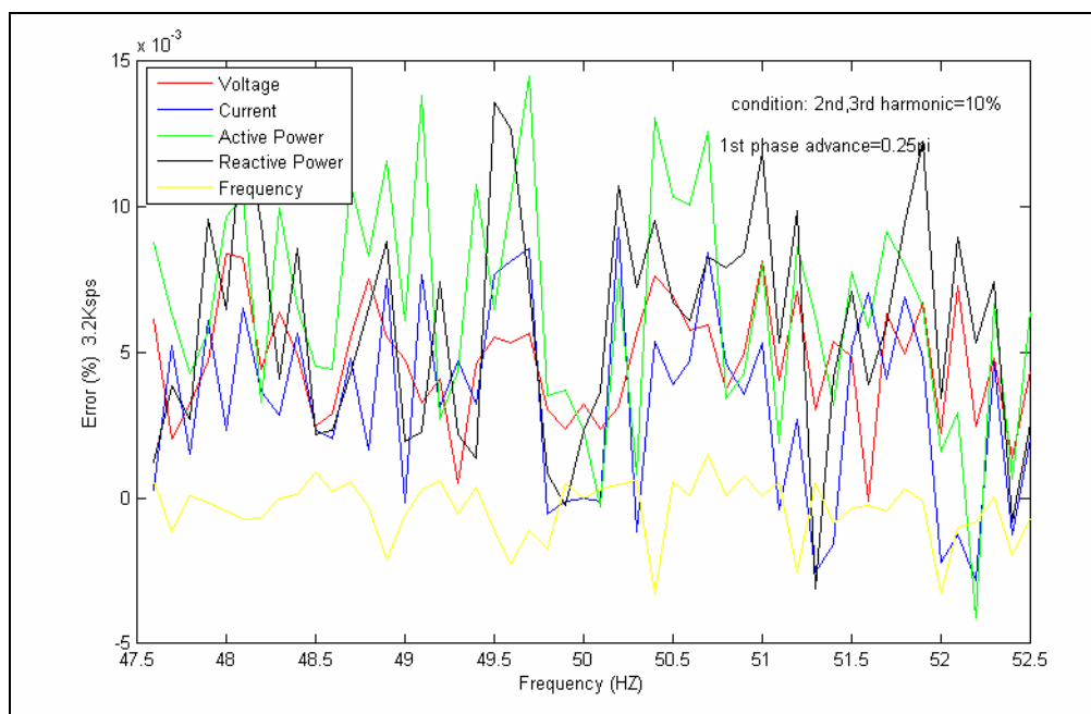
FIGURE C-6: Calculation Error Analysis After The Frequency Offset Compensation.
