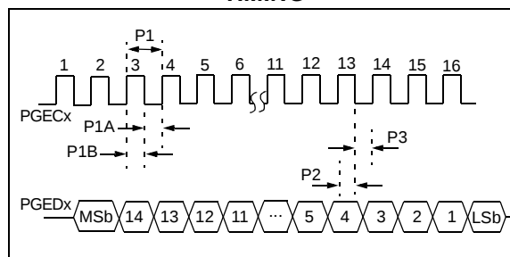
FIGURE 6-1: PROGRAMMING EXECUTIVE SERIAL TIMING
