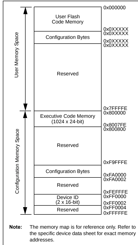
FIGURE 2-2: PROGRAM MEMORY MAP
