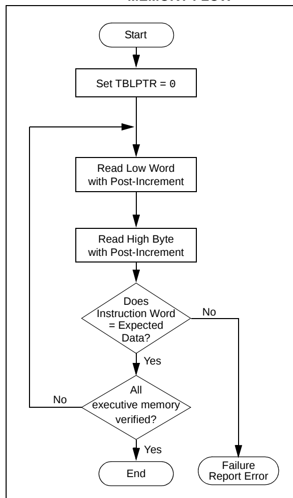
FIGURE 5-4: VERIFY EXECUTIVE MEMORY FLOW
