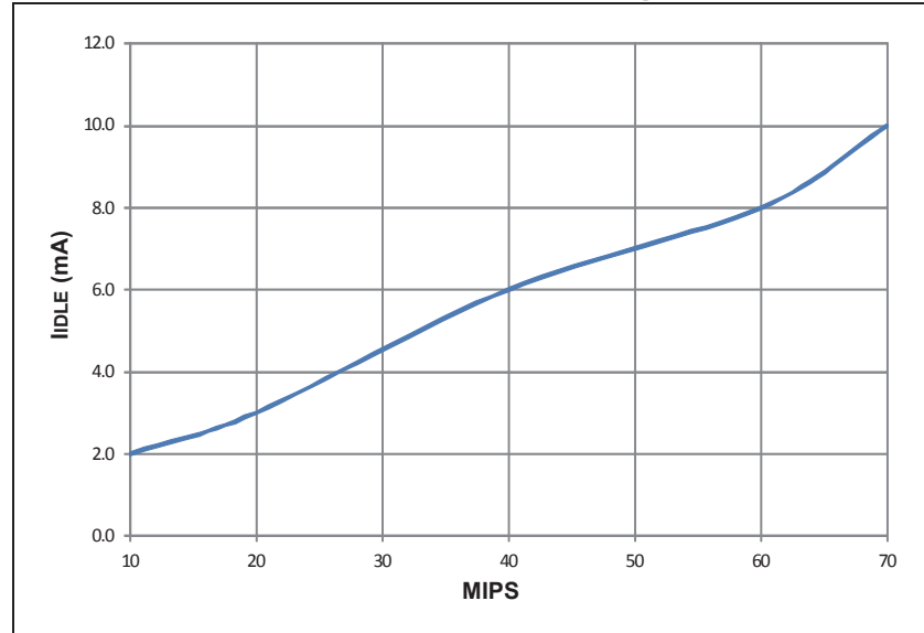
FIGURE 31-8: TYPICAL I_{IDLE} CURRENT @ V_{DD} = 3.3V , +25°C
