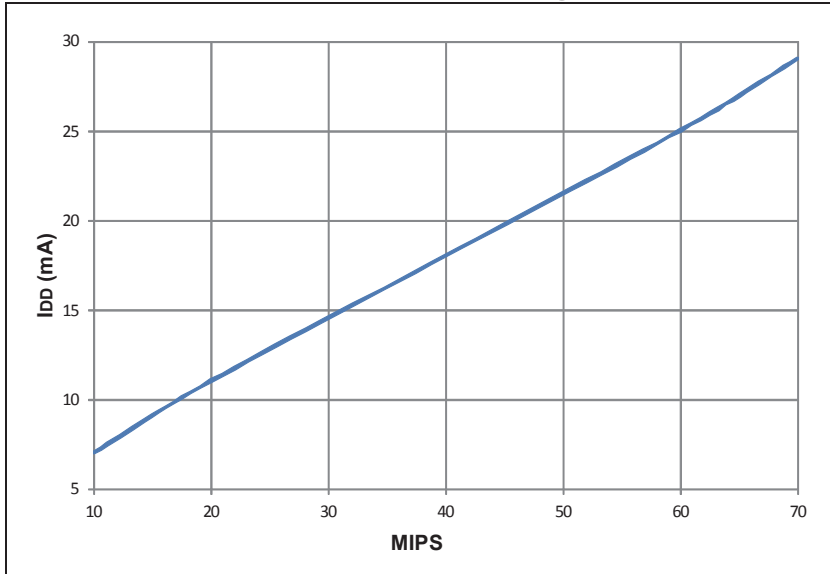
FIGURE 31-6: TYPICAL I_{DD} CURRENT @ V_{DD} = 3.3V , +25°C
