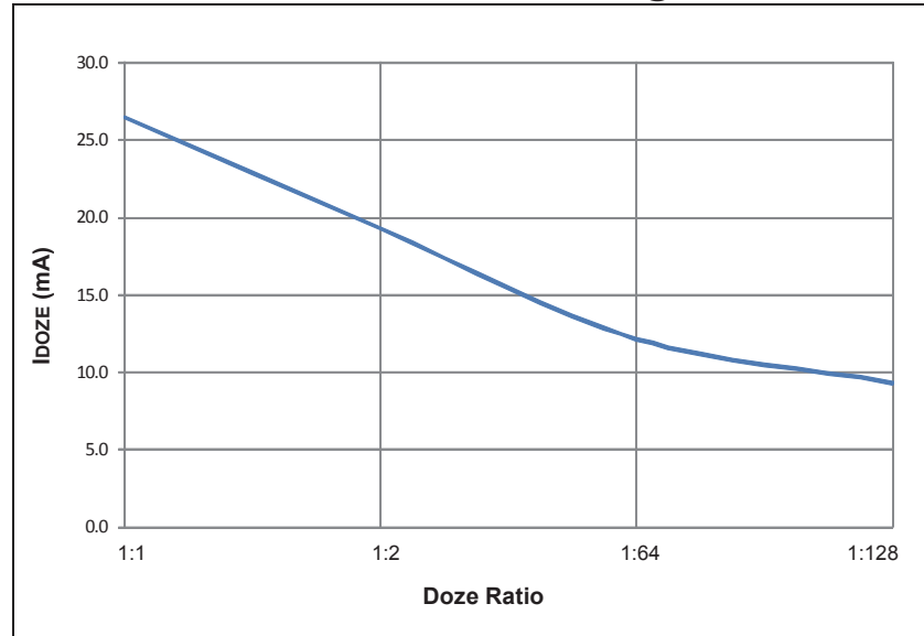
FIGURE 31-7: TYPICAL I_{DOZE} CURRENT @ V_{DD} = 3.3V , +25°C
