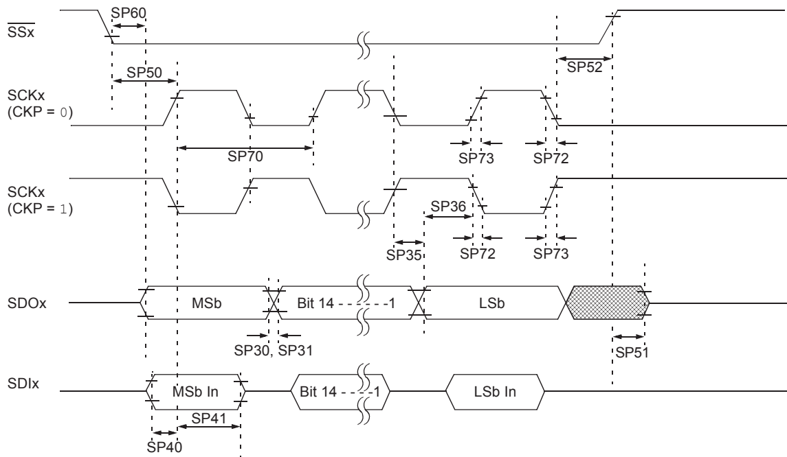
FIGURE 30-15: SPI1, SPI2 AND SPI3 SLAVE MODE (FULL-DUPLEX, CKE = 1, CKP = 0, SMP = 0) TIMING CHARACTERISTICS (1,2)
