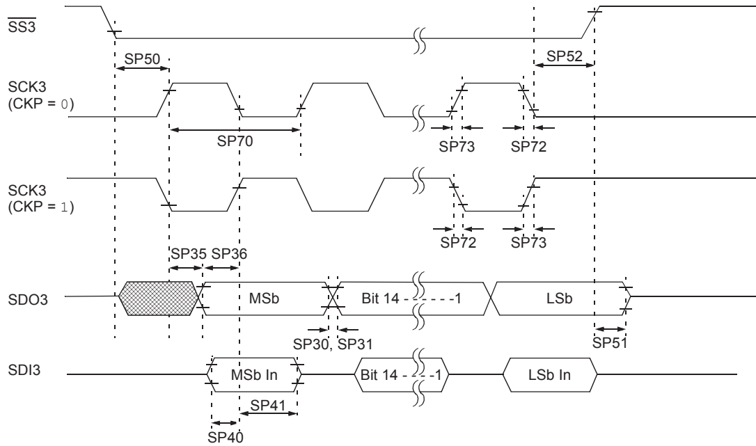
FIGURE 30-25: SPI3 SLAVE MODE (FULL-DUPLEX, CKE = 0, CKP = 1, SMP = 0) TIMING CHARACTERISTICS (1,2)
