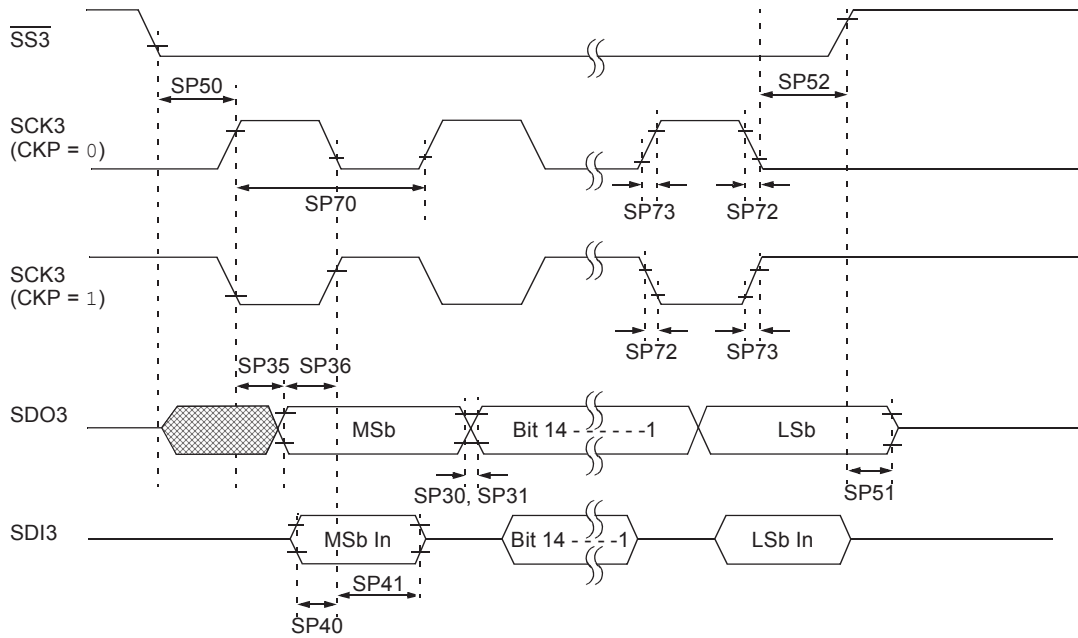
FIGURE 30-26: SPI3 SLAVE MODE (FULL-DUPLEX, CKE = 0, CKP = 0, SMP = 0) TIMING CHARACTERISTICS (1,2)
