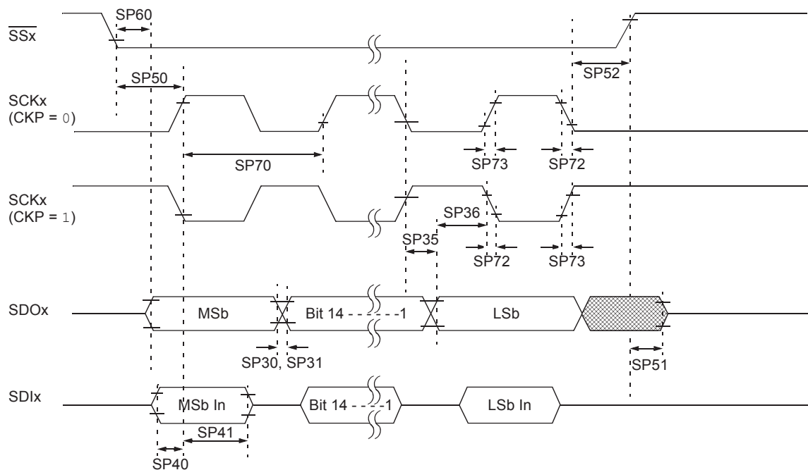
FIGURE 30-16: SPI1, SPI2 AND SPI3 SLAVE MODE (FULL-DUPLEX, CKE = 1, CKP = 1, SMP = 0) TIMING CHARACTERISTICS (1,2)
