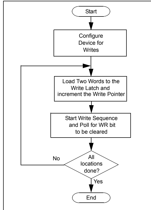
FIGURE 5-3: PROGRAM CODE MEMORY FLOW
