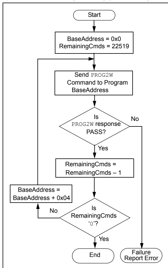
FIGURE 4-4: FLOWCHART FOR DOUBLE WORD PROGRAMMING
