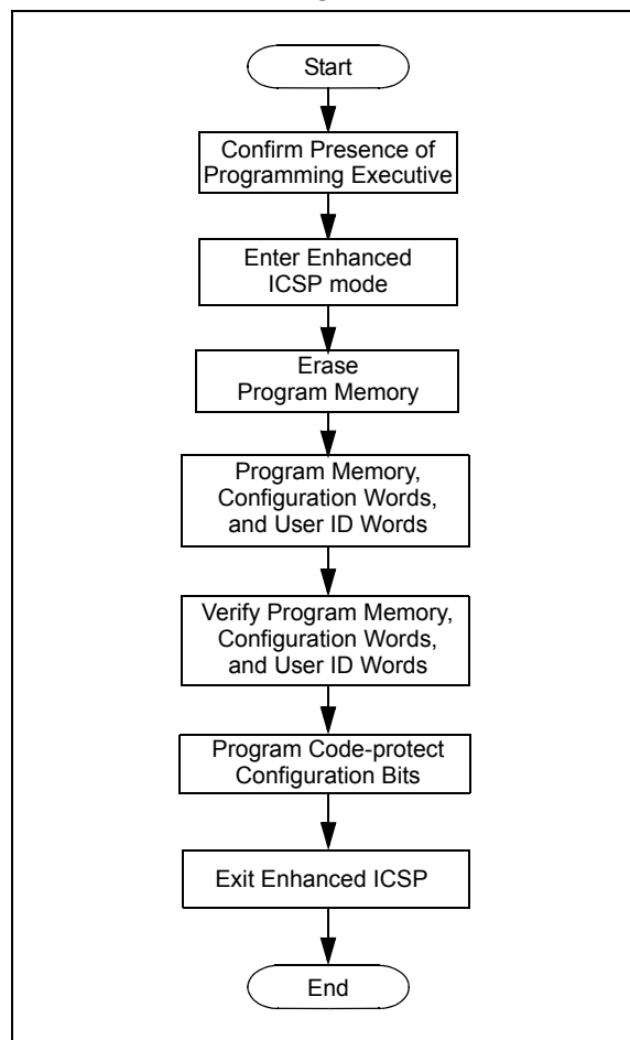
FIGURE 4-1: HIGH-LEVEL ENHANCED ICSP™ PROGRAMMING FLOW
